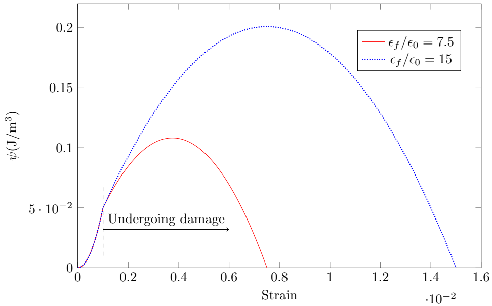
Figure 16: Variation of \psi with strain for different values of k = \epsilon_f/\epsilon_0 .
