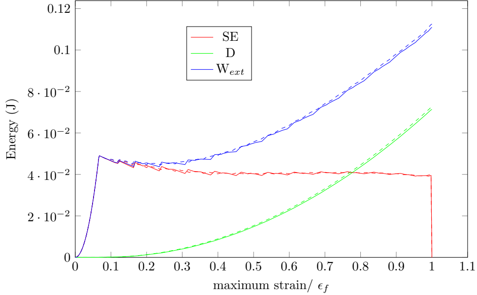
Figure 18: Evolution of different energies plotted as a function of ratio of the maximum strain in the body at each time to \epsilon_f . Here, \ell_{c0} = 0.1 m. The solid and the dashed lines indicate the results when 35 and 55 elements, respectively, are used.
