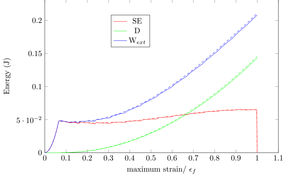
Figure 17: Evolution of different energies plotted as a function of ratio of the maximum strain in the body at each time to \epsilon_f . Here, \ell_{c0} = 0.2 m. The solid and the dashed lines indicate the results when 35 and 55 elements, respectively, are used.
