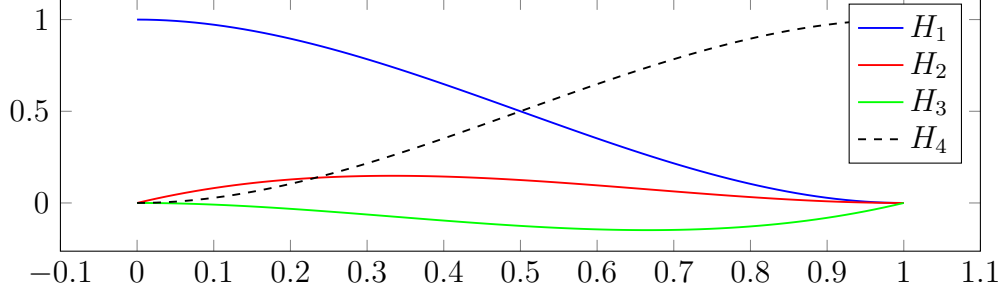
Figure 1: The Hermite polynomial shape functions for an element of unit length.
