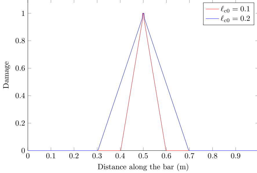
Figure 8: Damage profile when the bar breaks for \ell_{c0} = 0.1 m and 0.2 m.
