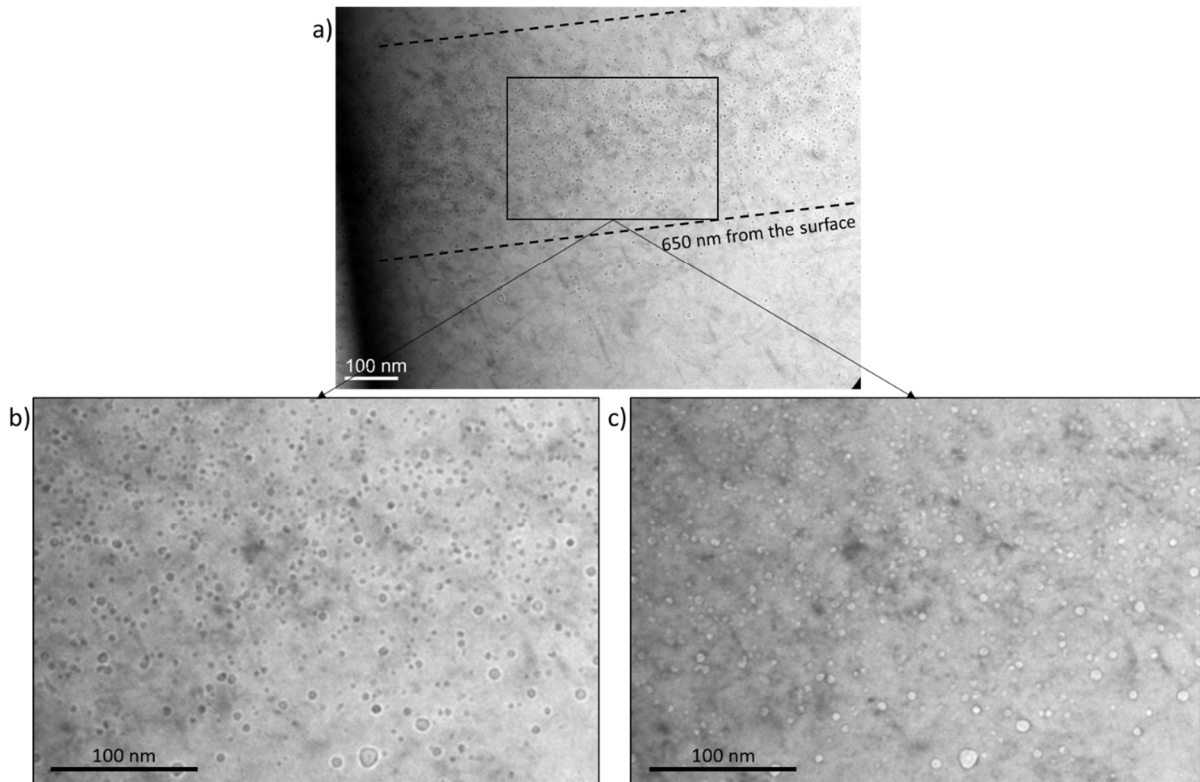
Figure 6 : Bright field TEM micrograph, a) and b) overfocused (+ 1 \mu\text{m} ), c) underfocused (- 1 \mu\text{m} ), evidencing cavities in JANNuS#2 type specimen. The free surface here is towards the bottom of the images.
