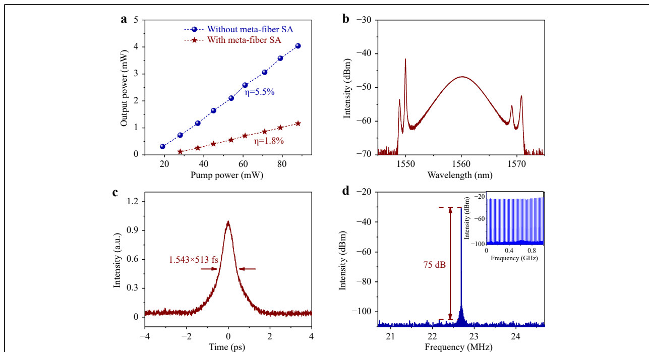
Fig. 4 Soliton mode-locking at 1.5 \mu\text{m} optical waveband incorporated with a plasmonic metafiber. a Averaged output power of a mode-locked fibre laser with the metafiber SA (red stars) and a cw laser without the metafiber SA (blue dots) as functions of the pump power. b Soliton pulse spectrum at pump power of 49 mW. c Autocorrelation trace of a single soliton at pump power of 58 mW. d RF spectrum of the soliton pulses with a scanning range of 5 MHz and a resolution of 300 Hz. The inset shows the RF spectrum of the soliton pulses with a scanning range of 1 GHz and a resolution of 10 KHz.
