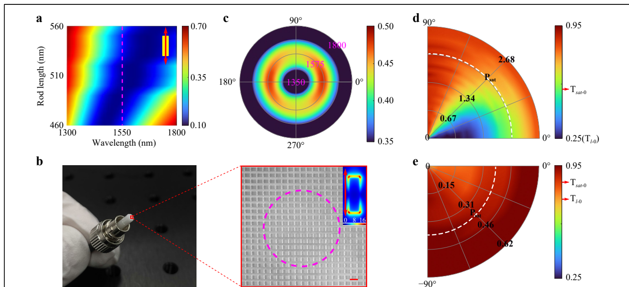
Fig. 2 Nanocharacterisation of the plasmonic metafibers. a Calculated transmission spectra of the Au nanorod arrays with varying rod lengths. The rod width is 160 nm and the height is 50 nm. The longitudinal and transverse periods remain constant at 750 nm. The excitation polarisation is parallel to the long axis of the nanorods. The pink dashed line indicates the spectral wavelength of 1550 nm. b Photograph of the fabricated metafiber by using EBL and the corresponding SEM image in the fibre core region. The scale bar represents 800 nm. The dashed pink circle indicates the boundary of the fibre core. The inset shows the fundamental electrical field distribution of the nanorod array (taking the periodic conditions into account). The red arrow represents the incident polarisation. The horizontal lines between two rows of nanorods presented in the SEM figure were caused by the charge accumulations during the SEM observations. c Experimental polarimetric extinction spectra of the plasmonic metafiber. The polar coordinates (\lambda, \theta) represent the spectral wavelength and the polarisation angle of the incident light. The colour contrast represents the extinction level of the metafiber. d, e Power- and polarisation-dependent nonlinear transmission of a nanorod array in on-resonance (using 1550 nm fs laser) and off-resonance (using 1950 nm fs laser) excitation conditions. The polar coordinates (P, \theta) represent the averaged power in the focus and the polarisation angle of the incident light. The colour contrast represents the transmission level of the nanorod array. The white dashed curves represent averaged saturation powers. T_{l-0} and T_{sat-0} denote the transmission levels at \theta = 0^\circ in the linear absorption regime and once absorption is saturated, respectively.
