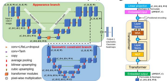
Figure 2. An overview of the CMF-Net with the schematic diagram of transformer modules is shown on the right side.
