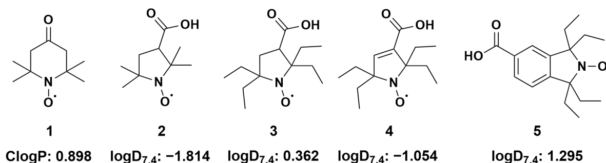
Figure 1. Structural formulas of investigated nitroxides and corresponding ClogP (calculated n-octanol/water partition coefficient) and logD 7.4 (distribution coefficients at pH 7.4). (1) 2,2,6,6-tetramethyl-4-oxo(piperidine-1-yloxy) radical (TEMPONE) (2) 3-carboxy-2,2,5,5-tetramethyl-1-pyrrolidinyloxy; (3) 3-carboxy-2,2,5,5-tetraethyl-1-pyrrolidinyloxy; (4) 3-carboxy-2,2,5,5-tetraethyl-1-pyrrolinyloxy; (5) 5-carboxy-1,1,3,3-tetraethyl-2-isoindolyloxy; Details of calculations are given in the Material and Methods section and in Supplementary Table S1.
