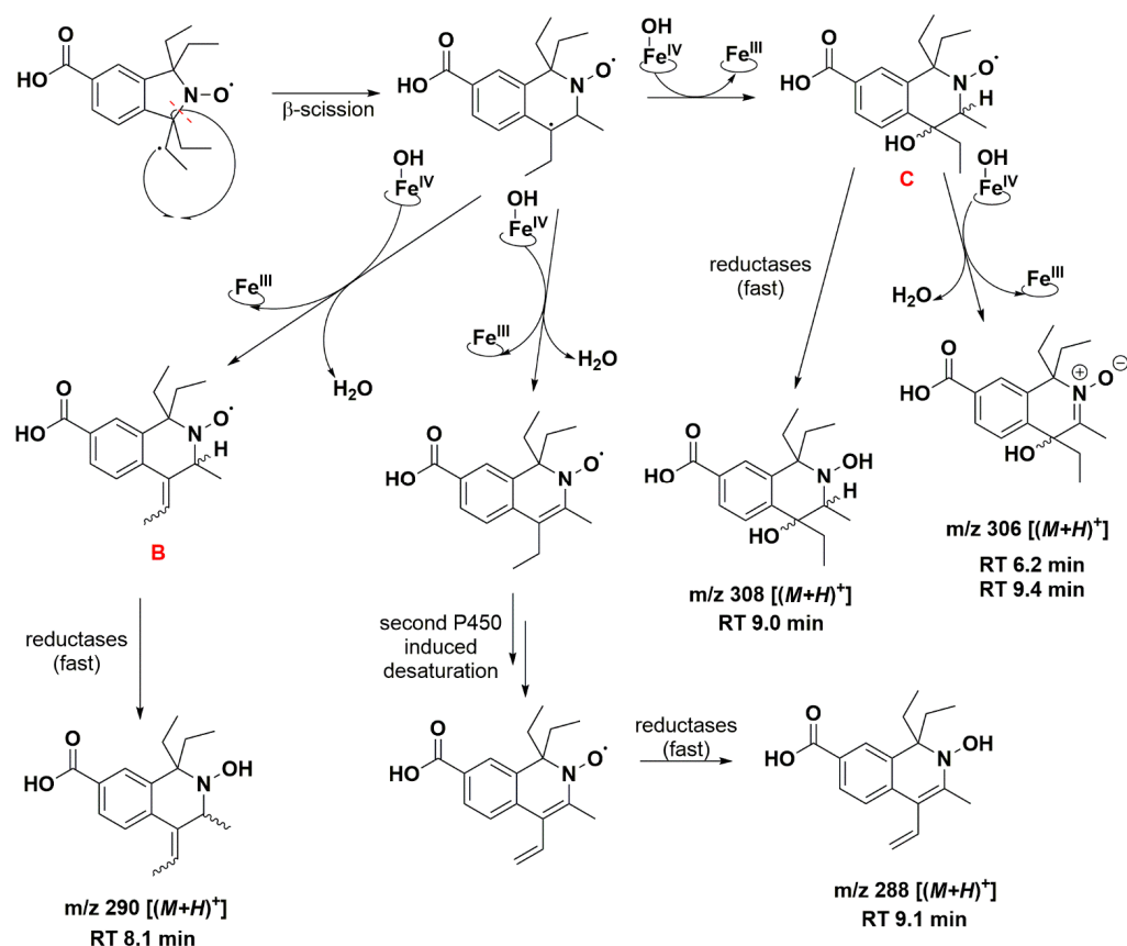
Figure 9. Proposed reaction pathway in the aerobic transformation of nitroxide 5 by RLM and NADPH, part II. Explicit hydrogens attached to carbon atoms in structures B and C correspond to potential origin of the coupling seen in the EPR spectra. Only one possible isomer is presented at each stage for the sake of clarity. The given RT values correspond to the reconstructed chromatograms of the principal ions obtained in HRMS study and were characterized by a delay of 0.2 min compared to the UV-Vis detection (see Figure 7).
