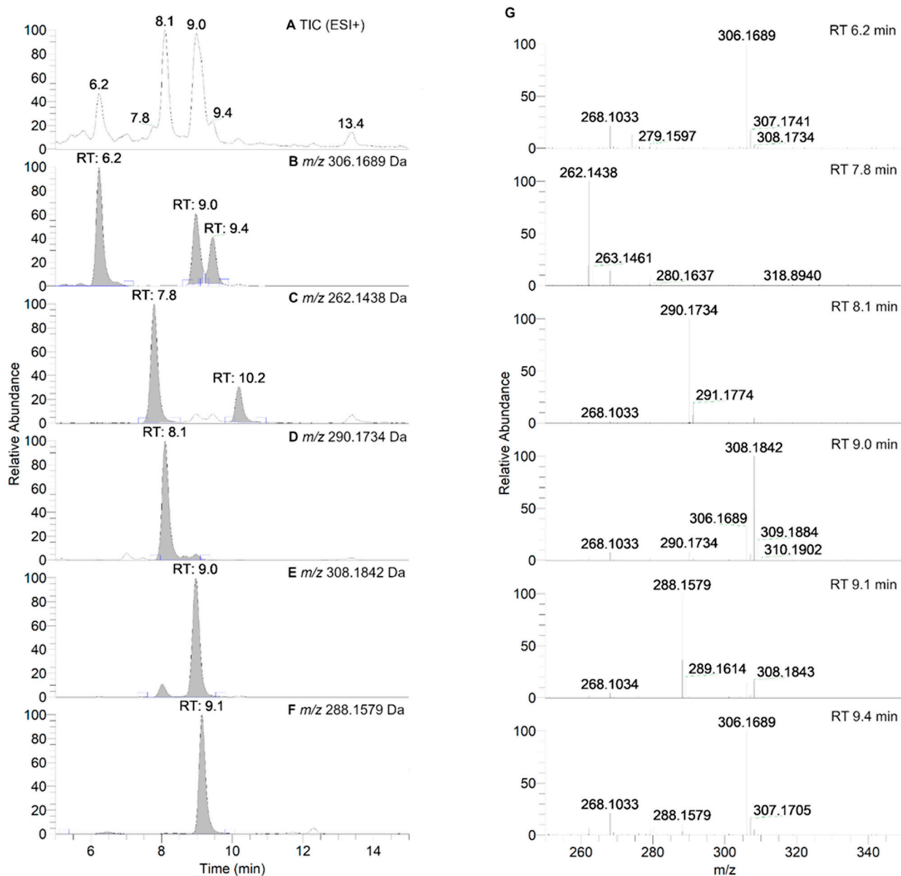
Figure 7. HPLC-HRMS study of nitroxide 5 (300 \mu\text{M} ) incubated with RLM (7.8 \text{mg}\cdot\text{mL}^{-1} protein, 30 \mu\text{M} P450) supplemented with NADPH (2 mM) in potassium phosphate buffer (100 mM; \text{pH} 7.4) upon aerobic conditions after 60 min. ( Panel A ) shows the TIC chromatogram in ESI + . ( Panels B–F ) display reconstructed chromatograms of the principal ions in ESI + mode identified at m/z = 306.1689 , 262.1438, 290.1734, 308.1842, and 288.1579 Da, respectively. ( Panel G ) represents the HRMS spectra of the peaks at retention times (RT) = 6.2, 7.8, 8.1, 9.0, 9.1 and 9.4 min. Peaks in TIC chromatograms were observed with a delay of 0.2 min compared to the UV-Vis detection.
