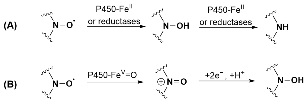
Figure 4. Proposed transformations of nitroxides: (A) 1 (TEMPONE) and 5 by P450 under anaerobic conditions; (B) 1 (TEMPONE) and 2 when incubated with RLM and NADPH under aerobic conditions.
