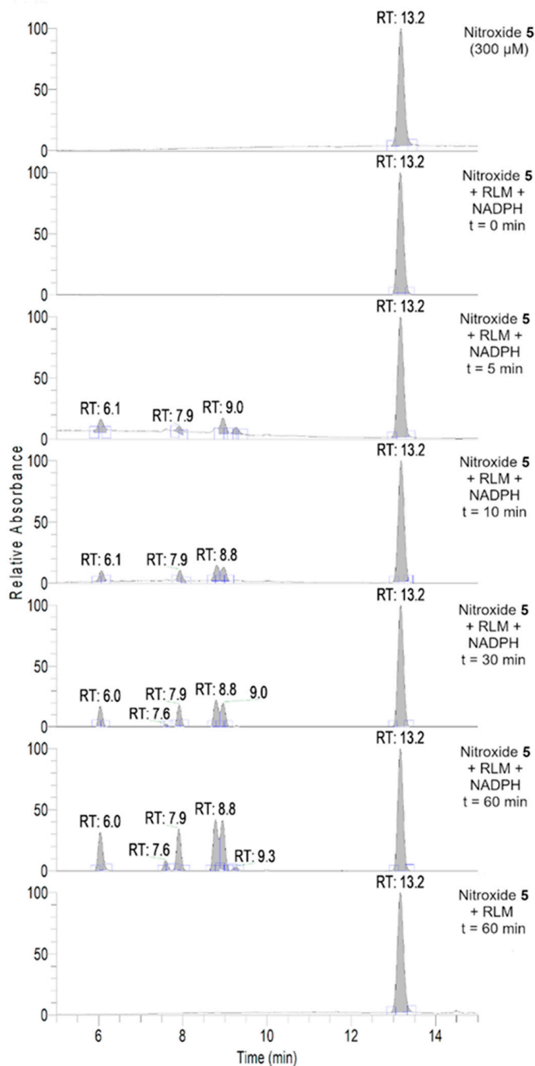
Figure 6. Total scan UV-Vis chromatograms of incubations of nitroxide 5 (300 μM) with RLM (30 μM of P450) with and without NADPH (2 mM) in potassium phosphate buffer (0.1 M, pH 7.4) in the presence of oxygen at 21 °C at different time points. Samples were prepared and analyzed as described in the experimental section.
