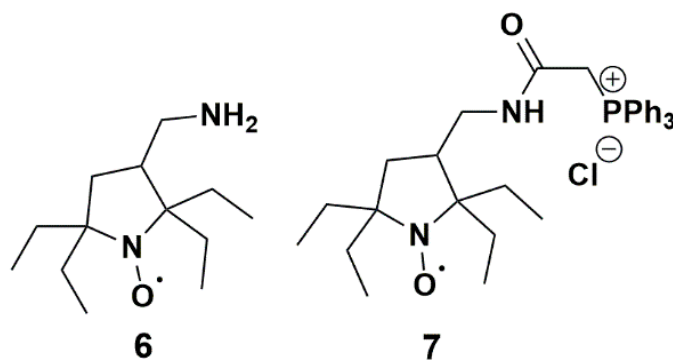
Figure 12. Pyrrolidine nitroxides tested by Kirilyuk et al.; (6) 3-(aminomethyl)-2,2,5,5-tetraethylpyrrolidine-1-oxyl; (7) 3-(2-(triphenylphosphonio)acetamidomethyl)-2,2,5,5-tetraethylpyrrolidine-1-oxyl chloride.
