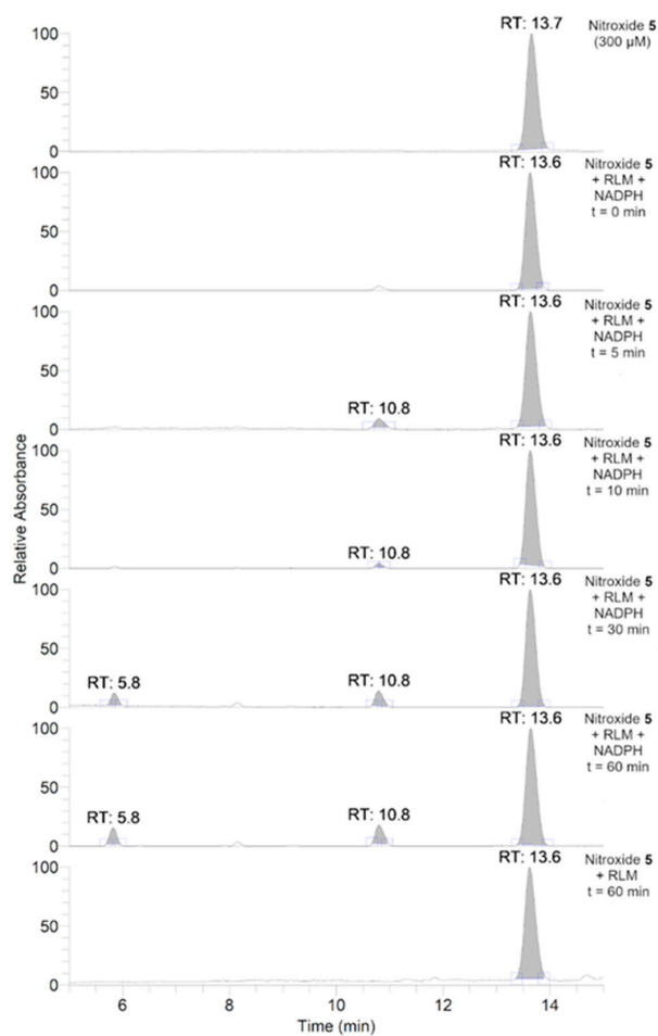
Figure 2. Total scan UV-Vis chromatograms of the incubations of nitroxide 5 (300 μM) in RLM (7.8 mg·mL -1 protein, 30 μM P450) with or without NADPH (2 mM) in potassium phosphate buffer (100 mM, pH 7.4) upon anaerobic conditions. Samples were prepared and analyzed as described in the experimental section.
