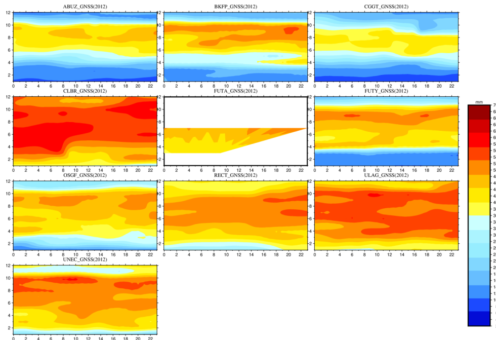
Figure 5. Sub-daily variation of GNSS PWV (mm) over 15 CORS for year 2012, plots are months against time (UTC hours)
