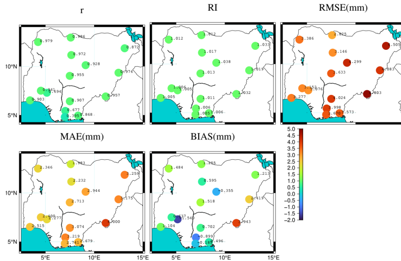
Figure 9. Statistical plot of sub-daily agreement of PWV from ERA5 and GNSS from 2012–2013
