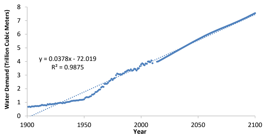
Figure 2. The global annual water demand in the period (1901–2100).
