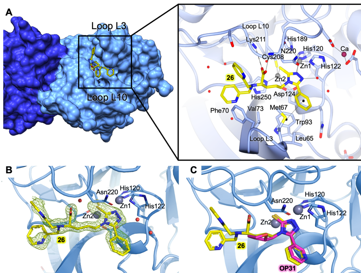
Figure 9. (A) NDM-1 (blue cartoon and carbon atoms; residues in sticks) in complex with compound 26 (in sticks, yellow carbons, PDB code 8A76), with detailed view of the interactions with NDM-1 residues (A, zoomed inset). (B) Omit map contoured at the 3- \sigma level. (C) Superposition of 26 (in sticks, yellow carbons) and the triazole-thione-based inhibitor OP31 (in sticks, fuchsia carbons) from PDB 6TGD. Zn ions and water molecules are displayed as grey and red spheres (arbitrary radius), respectively. In all figures, oxygen atoms are colored red, nitrogen blue and sulfur yellow.
