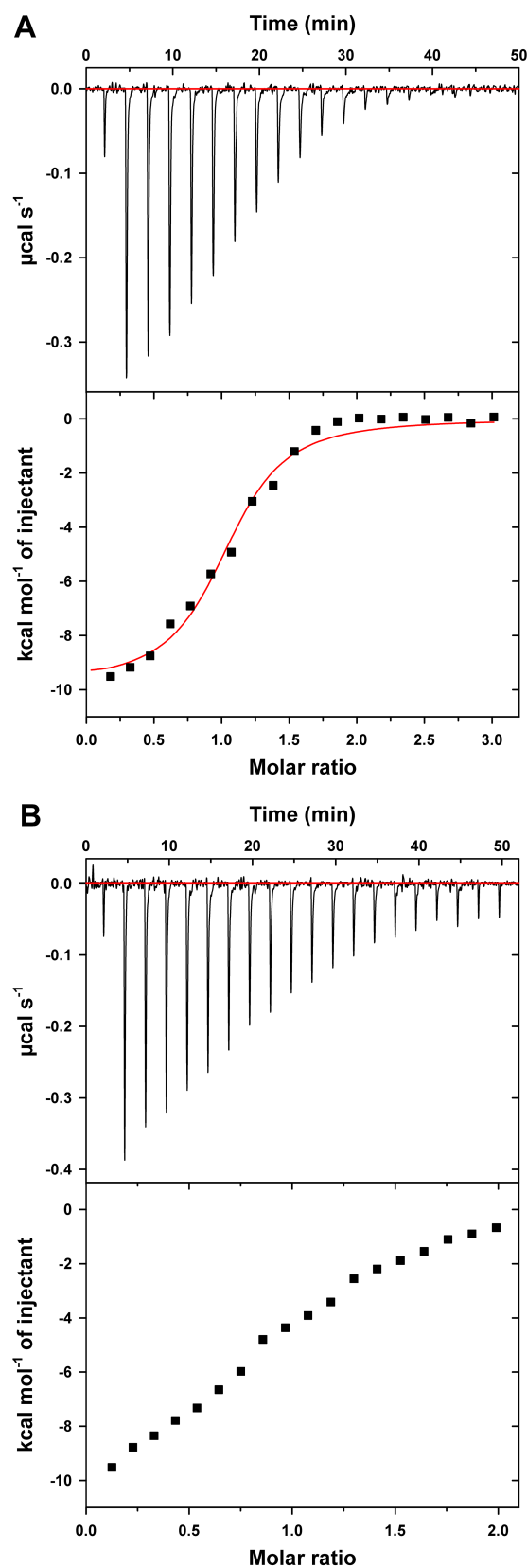
Figure 6. Isothermal titration calorimetry of VIM-2 by compounds 8 (A) and 26 (B) at 25 °C. Upper panel: exothermic microcalorimetric trace of compound injections into VIM-2 solution (19.0 µM). Lower panel: Wiseman plot of heat releases versus molar ratio of injectant/protein in the cell and nonlinear fit of the binding isotherm for n equivalent binding sites. The binding enthalpy corresponds to the amplitude of the transition curve, K_a is derived from the slope of the transition and the stoichiometry n is determined at the transition midpoint.
