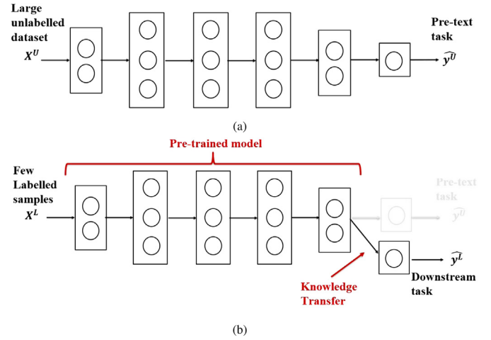
Fig. 5. A schematic view of the Self-Supervised Learning procedure (a): Pre-training phase in a self-supervised way, (b): Fine-tuning phase (supervised training on downstream tasks).
