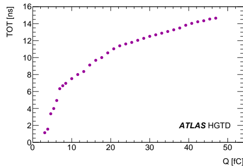
Figure 6.17: Time-over-threshold measured as a function of the injected charge.
