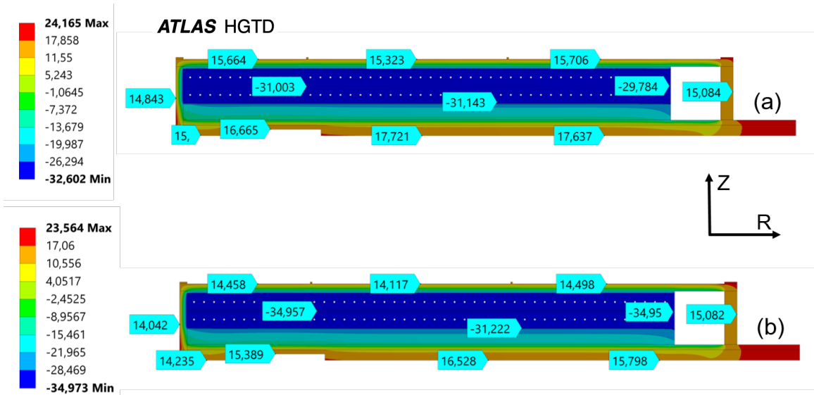
Figure 11.12: Temperature distribution within the FEA axisymmetric model of the detector assembly in the ATLAS experiment, with anti-condensation heaters powered on (front cover 80 \text{ W m}^{-2} , back cover 85 \text{ W m}^{-2} , outer ring 230 \text{ W m}^{-2} , inner ring 60 \text{ W m}^{-2} , total per end-cap 650 \text{ W} ). The dew point is set to 14^\circ\text{C} and the temperature distribution is plotted with detector units turned on at 0.35 \text{ W cm}^{-2} (a) and turned off (b).
