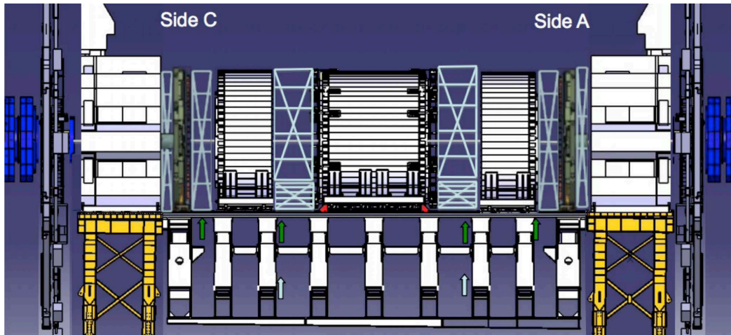
Figure 13.1: ATLAS in standard opening configuration.
