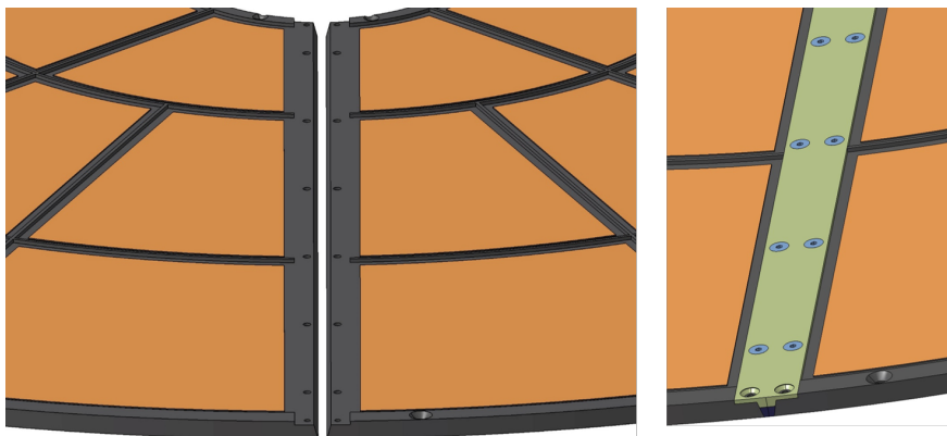
Figure 11.10: Detailed 3D view of the front cover junction connecting the two half moon parts. The central rod, on the right, is bolted on the two parts with trapezoidal elastomer gasket in place
