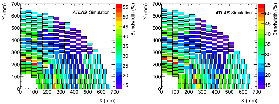
Figure 9.5: Readout bandwidth usage, in % of the capacity, for the expected number of average hits per ASIC from simulations with \langle \mu \rangle = 200 at a readout rate of 1 MHz. The usage is shown per sensor module in a quadrant of the first double sided layer. Left: Front layer. Right: Back layer. In regions corresponding to the readout rows 4-18, higher bit rate capacity is available (see text) resulting in lower bandwidth usage.
