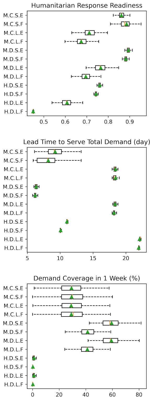
Figure 3. Box and whisker plots of the performance of the simulated HSC under different scenarios.
