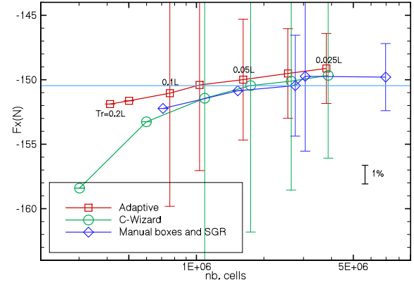
Figure 14: DTMB 5415, grid convergence and uncertainties for three series of meshes. The blue line represents the experimental result from [34].
