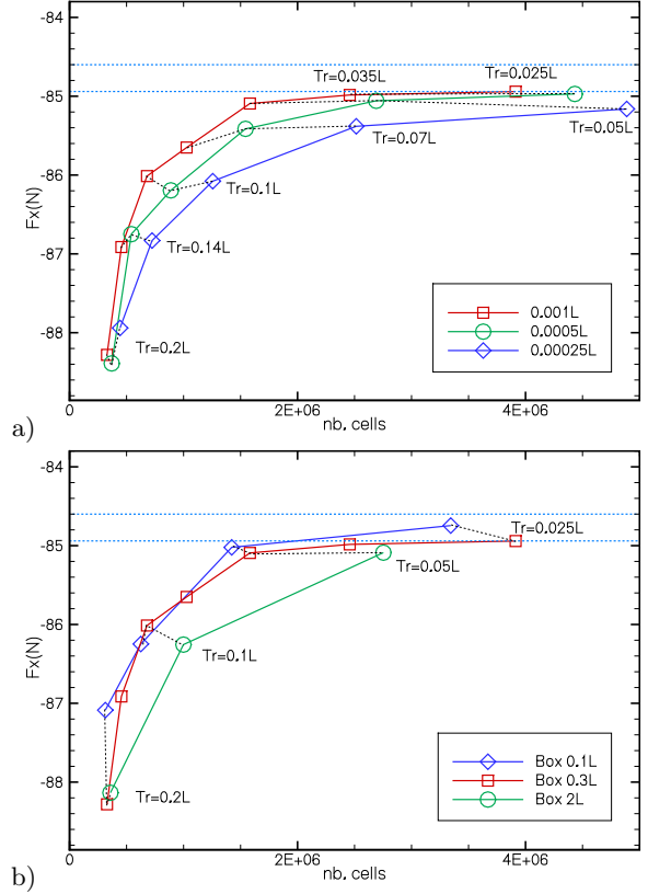
Figure 9: KCS, effect of the minimum cell size (a) and limiting box (b) on the resistance convergence with T_{rH} . The blue lines show the uncertainty interval of the experimental results [32].
