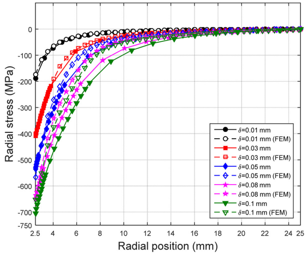
Fig. 5 Radial stresses—during loading
