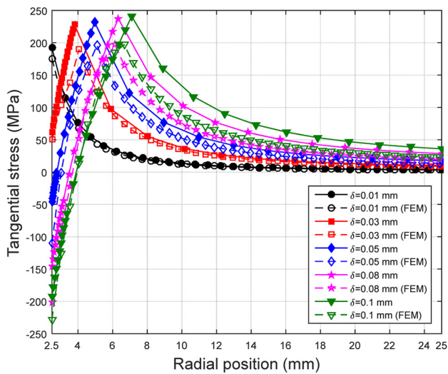
Fig. 7 Hoop stresses—during loading
