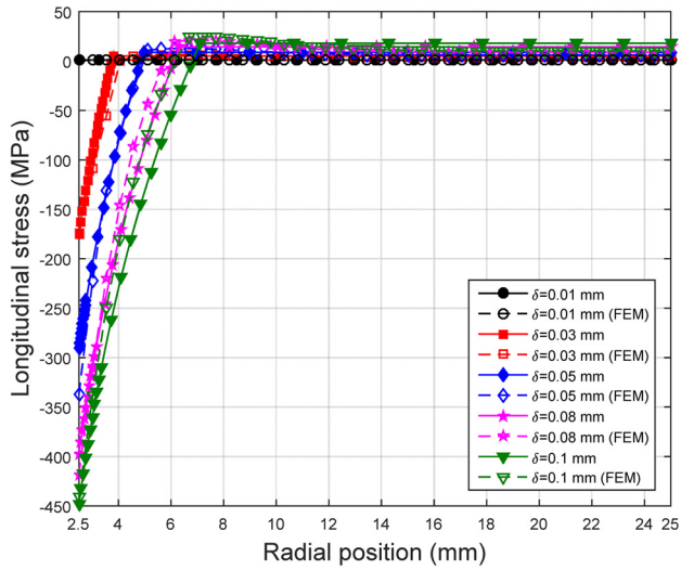
Fig. 6 Longitudinal stresses—during loading
