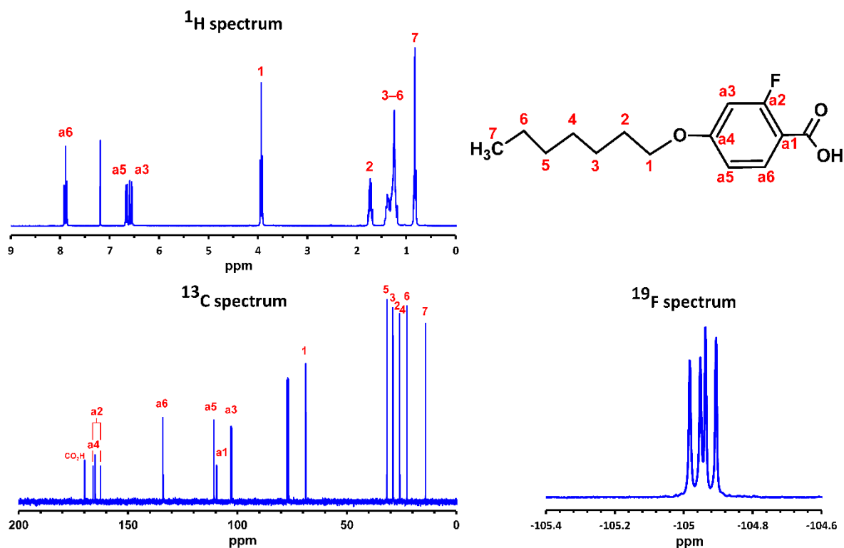
Figure S1. 1 H, 13 C and 19 F NMR spectra of 7OBAF in CDCl 3 solution.
