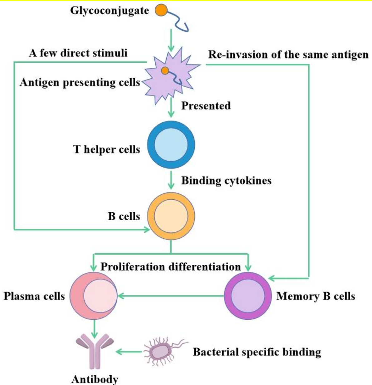
Fig. 16. Anti-bacterial mechanism of glycoconjugate vaccine.
