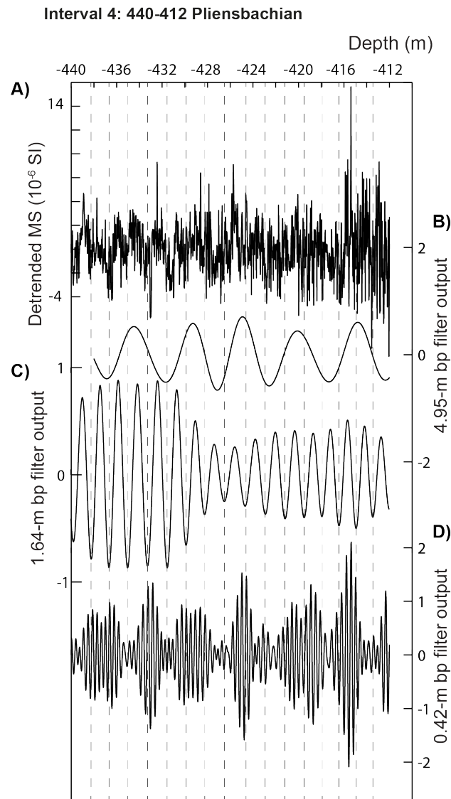
23 Fig. S2: Detail of the Pliensbachian interval showing the gradual variations of MS values. (A) 24 Detrended MS data from 440 to 412 m (Interval 4) with (B) cutoff frequencies 0.122 and
