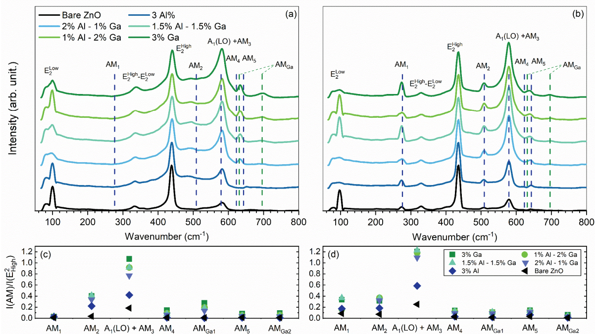
Figure 6. Raman spectra in the low wavenumber range for non-intentionally doped, Al- and Ga-doped ZnO NWs (a) before and (b) after thermal annealing at 400 °C for 1 hour under oxygen atmosphere as a function of the [\text{Ga}(\text{NO}_3)_3]/[\text{Zn}(\text{NO}_3)_2] and [\text{Al}(\text{NO}_3)_3]/[\text{Zn}(\text{NO}_3)_2] ratios in the chemical bath. (c,d) Intensity ratio of the AM over E_2^{\text{High}} lines of non-intentionally doped, Al- and Ga-doped ZnO NWs (c) before and (d) after thermal annealing at 400 °C for 1 hour under oxygen atmosphere as a function of the [\text{Ga}(\text{NO}_3)_3]/[\text{Zn}(\text{NO}_3)_2] and [\text{Al}(\text{NO}_3)_3]/[\text{Zn}(\text{NO}_3)_2] ratios in the chemical bath.
