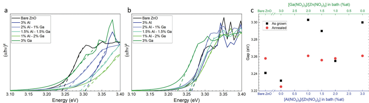
Figure 9. Tauc plots in non-intentionally doped, Al- and Ga-doped ZnO NWs (a) before and (b) after thermal annealing at 400 °C for 1 hour under oxygen atmosphere as a function of the [\text{Ga}(\text{NO}_3)_3]/[\text{Zn}(\text{NO}_3)_2] and [\text{Al}(\text{NO}_3)_3]/[\text{Zn}(\text{NO}_3)_2] ratios in the chemical bath. The dashed lines denote the fit of the linear portion to deduce the optical band gap energy from its intercept with the h\nu -axis. (c) Evolution of the optical band gap energy of non-intentionally doped, Al- and Ga-doped ZnO NWs before and after thermal annealing at 400 °C for 1 hour under oxygen atmosphere as a function of the [\text{Al}(\text{NO}_3)_3]/[\text{Zn}(\text{NO}_3)_2] and [\text{Ga}(\text{NO}_3)_3]/[\text{Zn}(\text{NO}_3)_2] ratios in the chemical bath.
