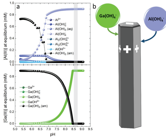
Figure 1. (a) Distribution of Al(III) and Ga(III) species at 85°C as a function of pH, as computed by Visual MINTEQ software. The NH_3 concentration was varied in the range of 0–1500 mM, while the Al(NO_3)_3 and Ga(NO_3)_3 concentrations were set to 0.9 mM. Each data point corresponds to the addition of 1 mM of NH_3 in the chemical bath. The grey rectangular area denotes the range of pH values experimentally measured at the end of the CBD process. (b) Schematic representing the adsorption processes of Al(OH)_4^- and Ga(OH)_4^- complexes on the charged surfaces of ZnO NWs during CBD. The sign of the surface electrical charge is taken at the pH value used during the CBD process, considering the PZC values of both the top polar c -planes and nonpolar m -plane sidewalls of ZnO NWs around 8.7 \pm 0.2 and 10.2 \pm 0.2 at room temperature. 34-35
