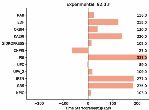
Fig. 11. Time of first core heat-up.
