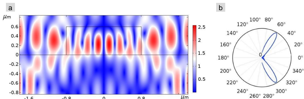
Figure 14: (a) Map of the modulus of the electric field (for TE polarization) in the near field at 604 nm for k_x = 6 \frac{2\pi}{D} . (b) Angular representation of the far field intensity (in a.u.) of the eigenmode.
