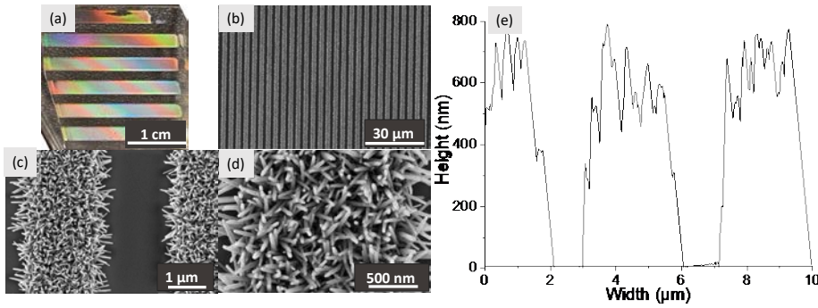
Figure 6: ZnO NW gratings on 2.5 \times 2.5 \text{ cm}^2 quartz substrate illustrated by macroscopic photography (a), low (b) to high magnification (d) SEM images, and AFM profile (e).
