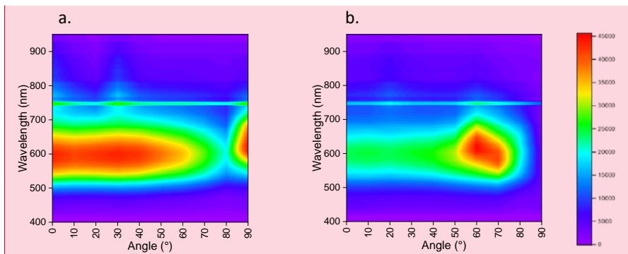
Figure 8: Room temperature ARPL map showing the evolution of the emission intensity with the wavelength and detection angle for (a) the ZnO coating and (b) the ZnO grating under 375 nm excitation
