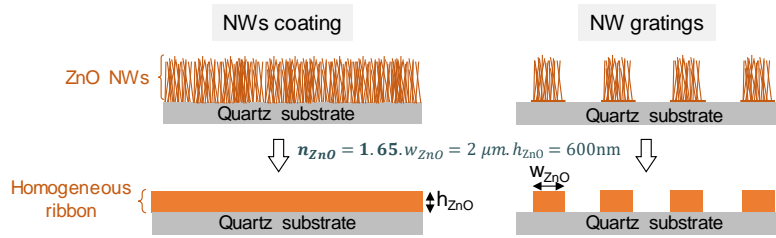
Figure 12: Schematic representation of the modelling of ZnO NW coating and grating by solid blocks. The main parameters used are noted in the center of the figure.
