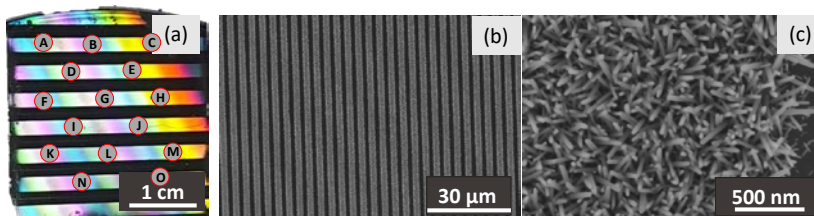
Figure 4: Large scale photograph (a) and SEM images at low (b) and high (c) magnifications of NW gratings elaborated on 3x3 cm 2 Si wafers after insulation at a 25 mW/cm 2 power. In the photo, the 15 areas noted A to O indicate where SEM images of Figure 5 have been considered.
