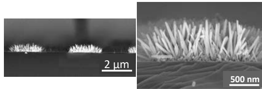
Figure 3: SEM cross section images of ZnO NW gratings on silicon obtained after insulation at a 25 mW/cm 2 power.
