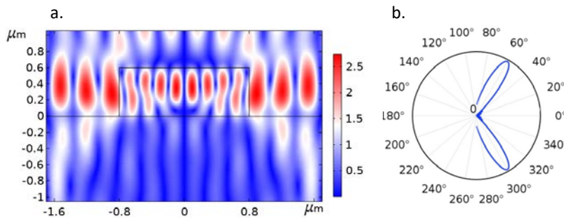
Figure 14: (a) Map of the modulus of the electric field (for TE polarization) in the near field at 604 nm for k_x = 6 \frac{2\pi}{D} . (b) Angular representation of the far field intensity (in a.u.) of the eigenmode.
