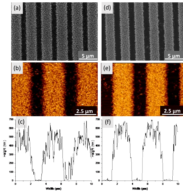
Figure 2: From top to bottom, SEM top view and AFM top view and profiles of ZnO NW gratings on silicon obtained after insulation at a power of 23.5 mW/cm 2 (a to c) and 25 mW/cm 2 (d to f).
