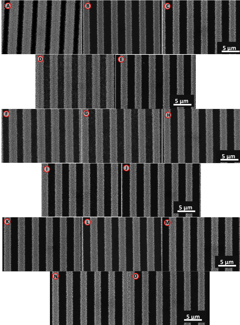
Figure 5: SEM top view mapping of ZnO NW gratings on a 3x3 cm 2 Si wafer obtained after insulation at a 25 mW/cm 2 power. The localization of areas A to O is depicted in Figure 4a.
