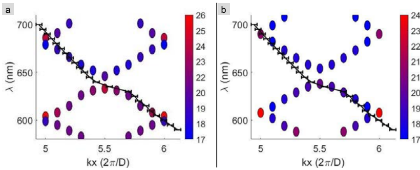
Figure 13: Colored circles: (a) and (b) are the theoretical dispersion relation for TE and TM polarizations, respectively, computed for ribbons of 1.6 \mu\text{m} width, 600 \text{ nm} height, and 4 \mu\text{m} grating period. The value of the quality factor corresponds to the color of the circles. The black curve is the experimental dispersion relation.
