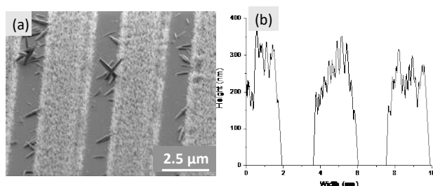
Figure 1: SEM Image showing the coexistence of linear NW gratings and big ZnO rods (a) and AFM profile of resulting gratings (b).
