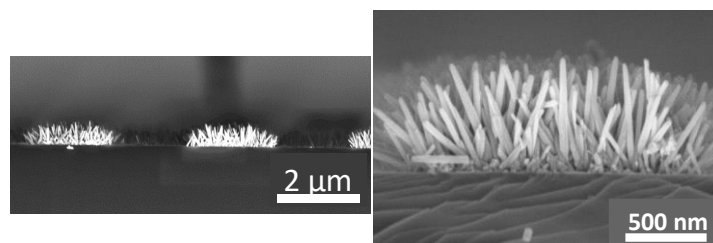
Figure 3: SEM cross section images of ZnO NW gratings on silicon obtained after insolation at a 25 \text{ mW/cm}^2 power.
