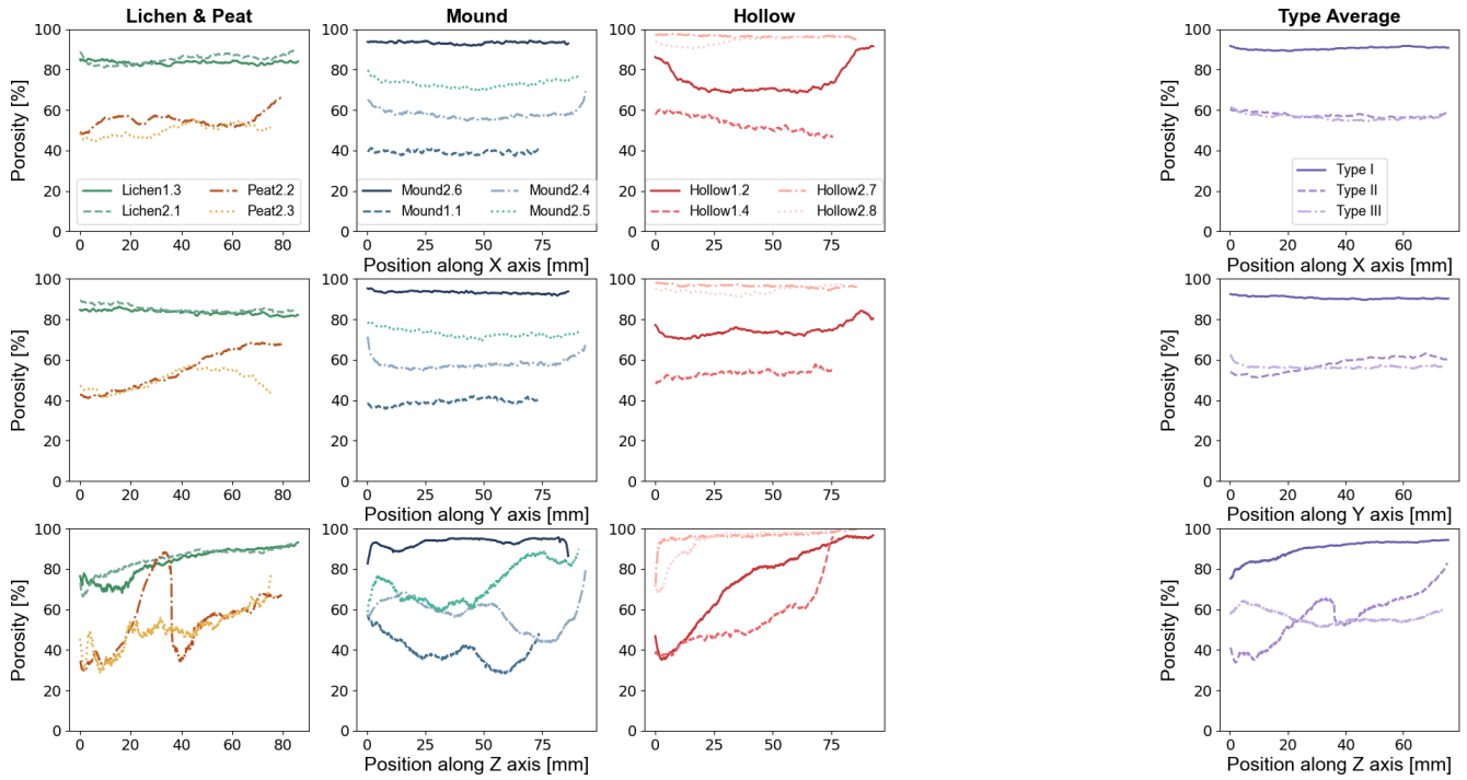
Figure 4. Planar porosity plot along the x , y and z axes for moss, lichen and peat samples. An averaged value is computed for each sample type, each color nuance representing each type. Type I : stable high-porosity profile samples, excluding border effects. Type II : low basal porosity, linearly increasing to the top of the sample. Type III : no specific trend observed in vertical porosity.
