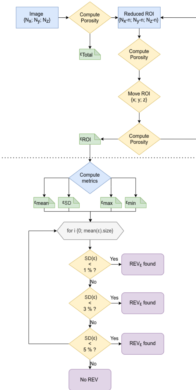
Figure 3. Flowchart of the representative elementary volume of porosity ( REV_{\epsilon} ) from a binarized image. For each sample, three thresholds are tested (5 %, 3 % and 1 % and standard deviation variation).
