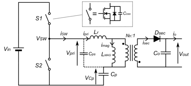
Figure 1 - 2L-AHBF schematic
