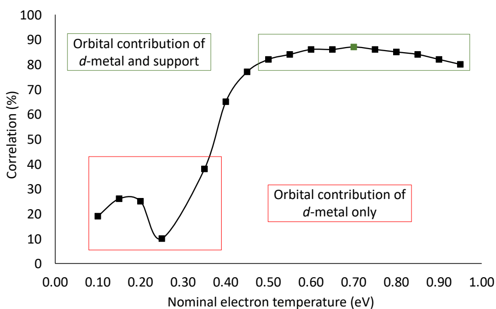
Figure 6. Correlation ( R^2 ) between the global softness evaluated as the inverse of the bandgap and the Fermi softness (y-axis) for nominal electron temperatures ranging between 0.10 and 0.95 eV (x-axis). A narrow weight function that mainly contains orbital contributions from the adsorbed metal shows a poor correlation with the global softness (pink). A larger weight function including both metal and support contributions substantially increases the correlation (green).
