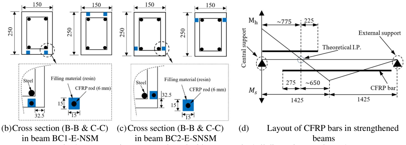
Fig. 2 Beam specimens strengthened with CFRP rods. (All dimensions are in mm)
