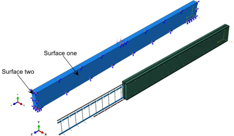
(b) Boundary conditions, steel Skelton and finite element mesh of quarter beam Fig.18: Detail and boundary condition of the FE beam (all dimension are in mm)
