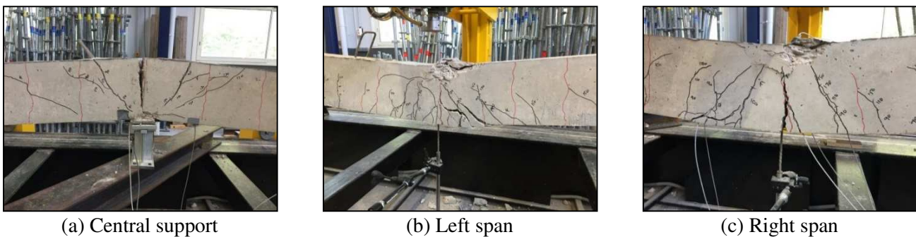
Fig.A.1: Failure mode of beam BC1-E-NSM-(0-2)
