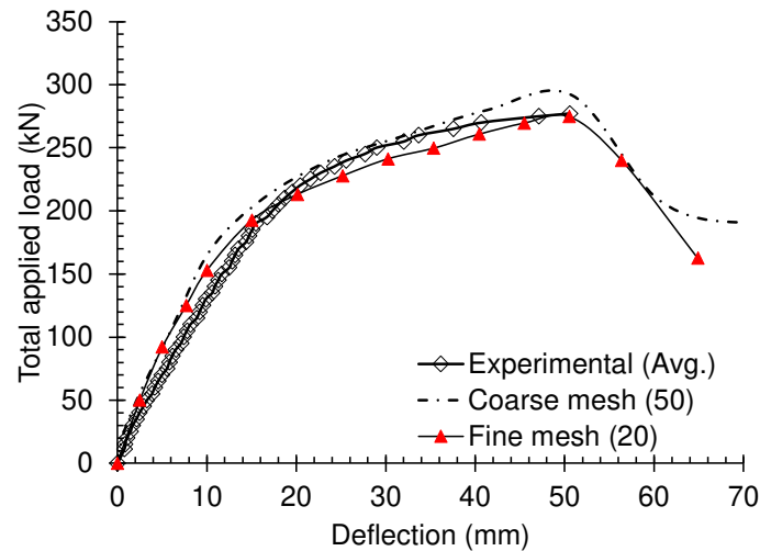
Fig.19: Effect of the mesh size
