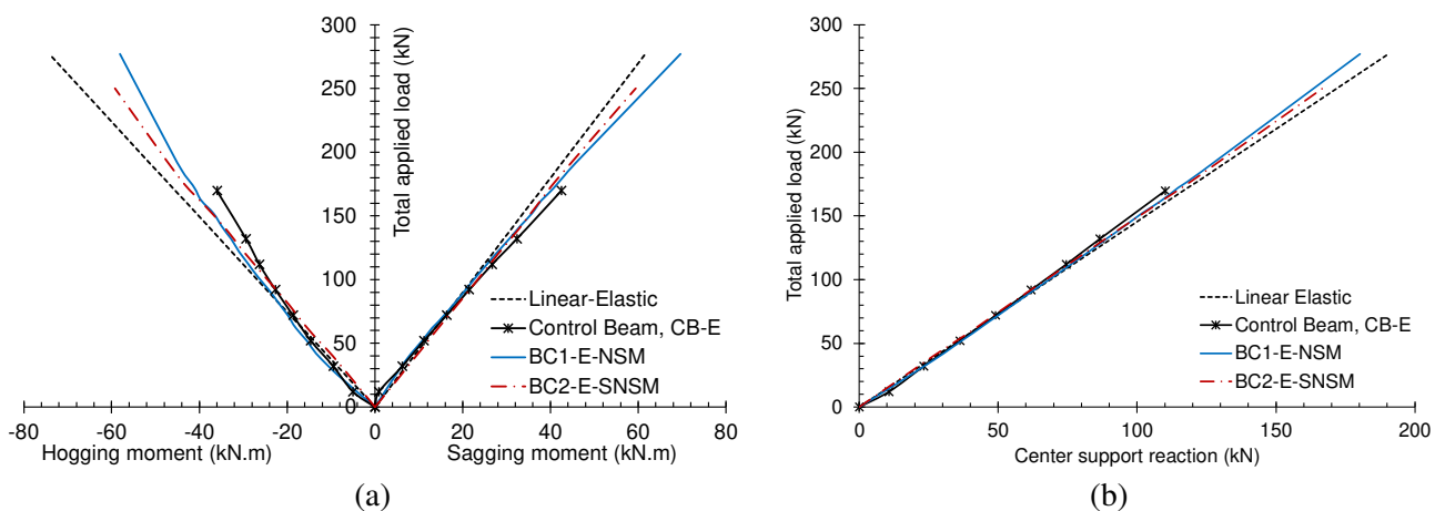
Fig.8: Total applied load versus (a) bending moment; (b) central support reaction
