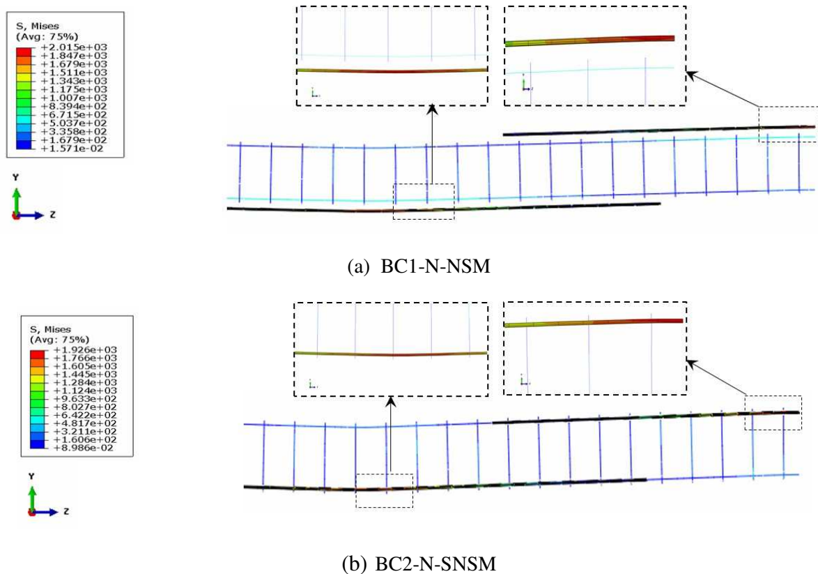
Fig. 23: The FEA (CZM) tensile stress of CFRP bars in the strengthened beams at the ultimate load level
