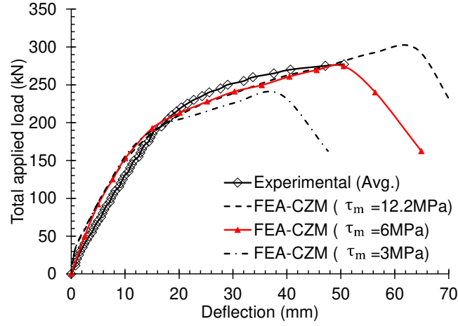
Fig.17: Comparison between the experimental results and FEA results with different value of maximum shear stress for beam BC1-E/N-NSM
