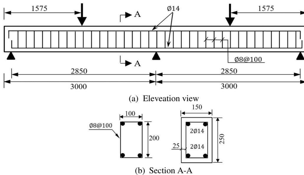
Fig. 1: Dimensions, steel layout as well as support and load arrangement of tested beams. (All dimensions are in mm)
