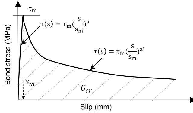
Fig.16: Bond slip law
