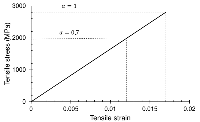
Fig.13: Constitutive model of CFRP reinforcement
