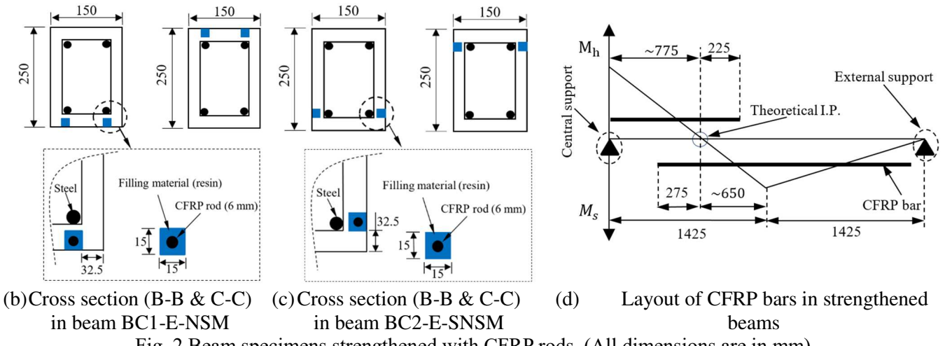
Fig. 2 Beam specimens strengthened with CFRP rods. (All dimensions are in mm)
