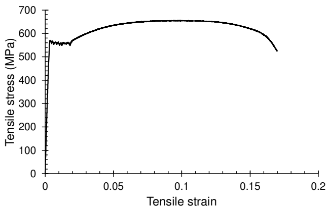
Fig.12: Constitutive model of steel reinforcement
