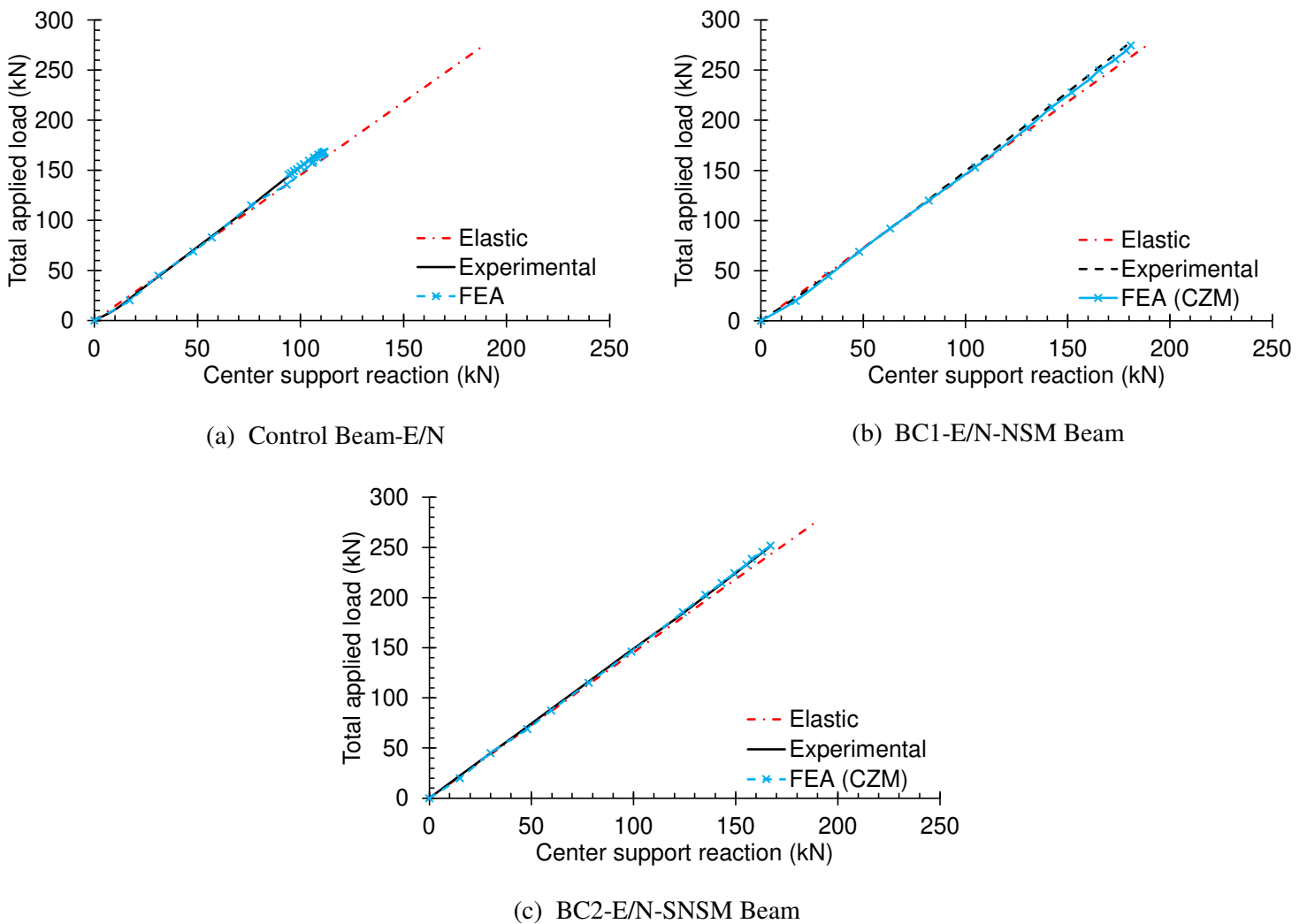
Fig. 22: The experimental and FEA results of central support reaction of tested beams
