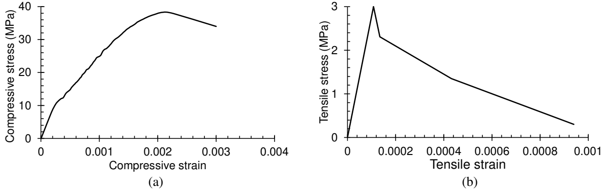
Fig.11: Response of concrete to uniaxial loading in (a) compression and (b) tension
