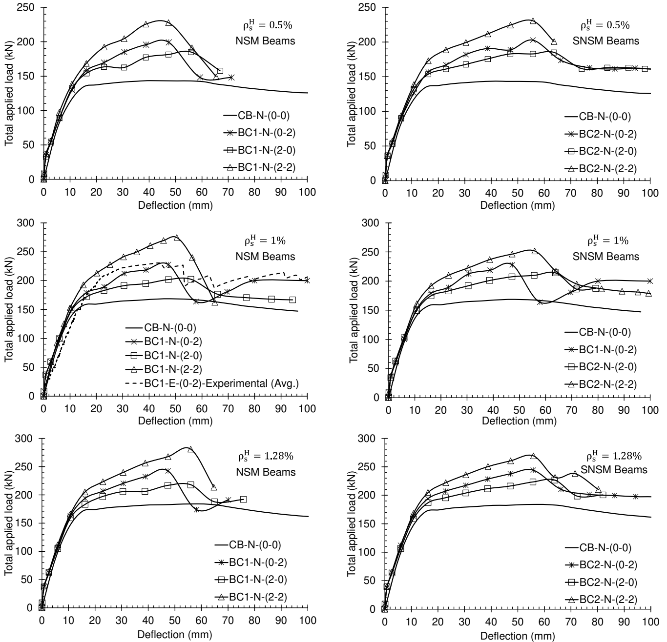
Fig.24. Load-deflection curves of FE beams
