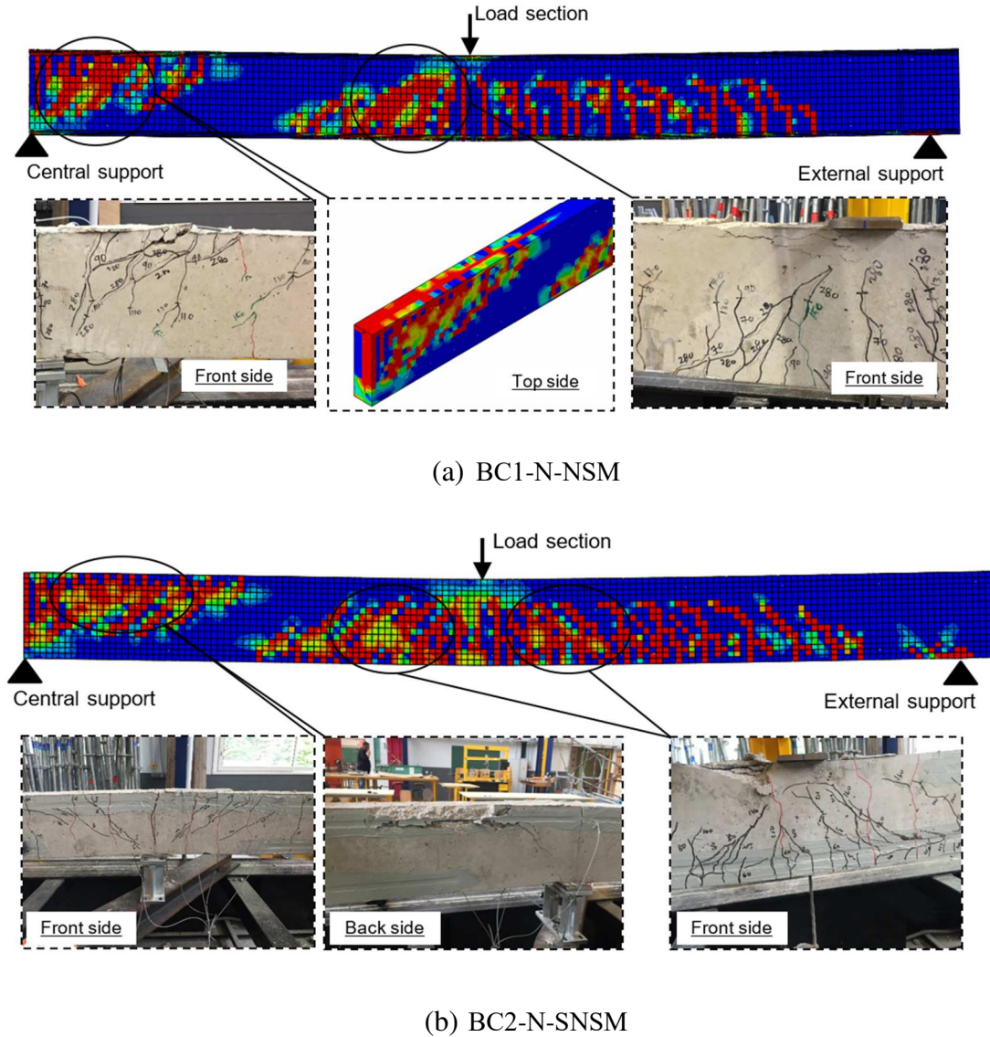
Fig. 21: Cracks maps and failure of strengthened beams
