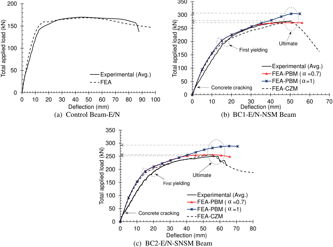
Fig. 20: The experimental and numerical load deflection curves of tested beams.
