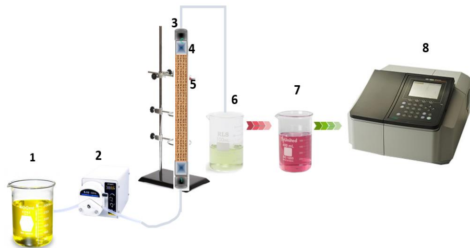
Figure 1. Schema of the experimental setup for the Cr(VI) fixed-bed adsorption. 1—Cr(VI) solution reservoir, 2—Peristaltic pump, 3—Cotton plugs, 4—Glass ball, 5—RPS fixed bed, 6—taken sample of Cr(VI), 7—Ready sample for analysis, 8—Spectrophotometer UV-Visible.
