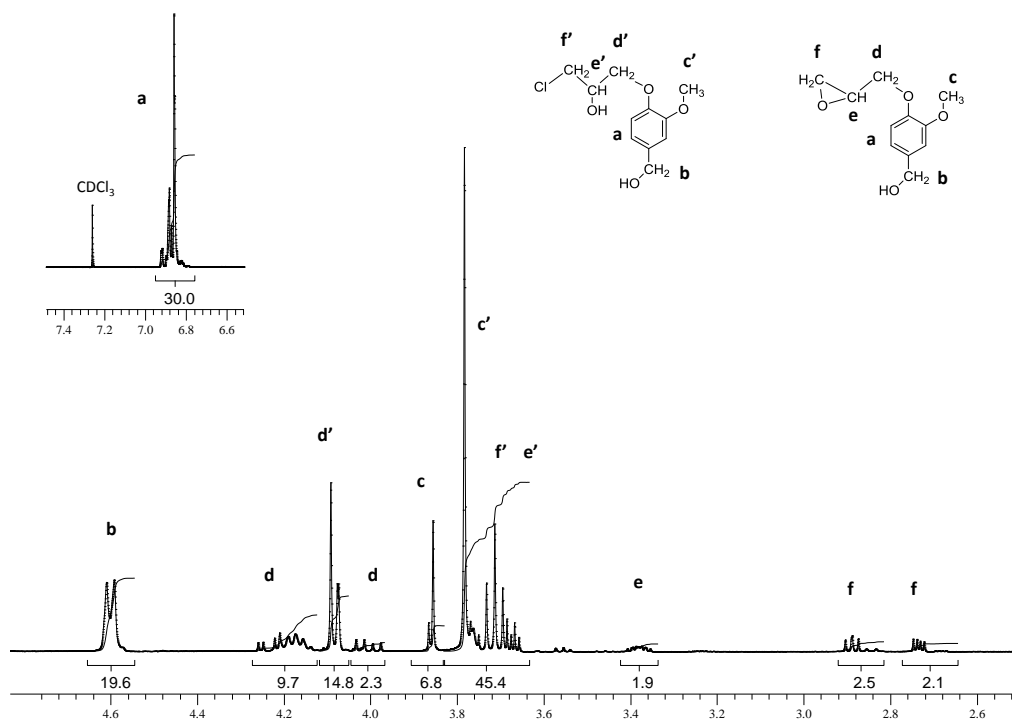
Figure 3: ^1\text{H} NMR spectrum of the vanillyl alcohol reaction with epichlorohydrin at room temperature
