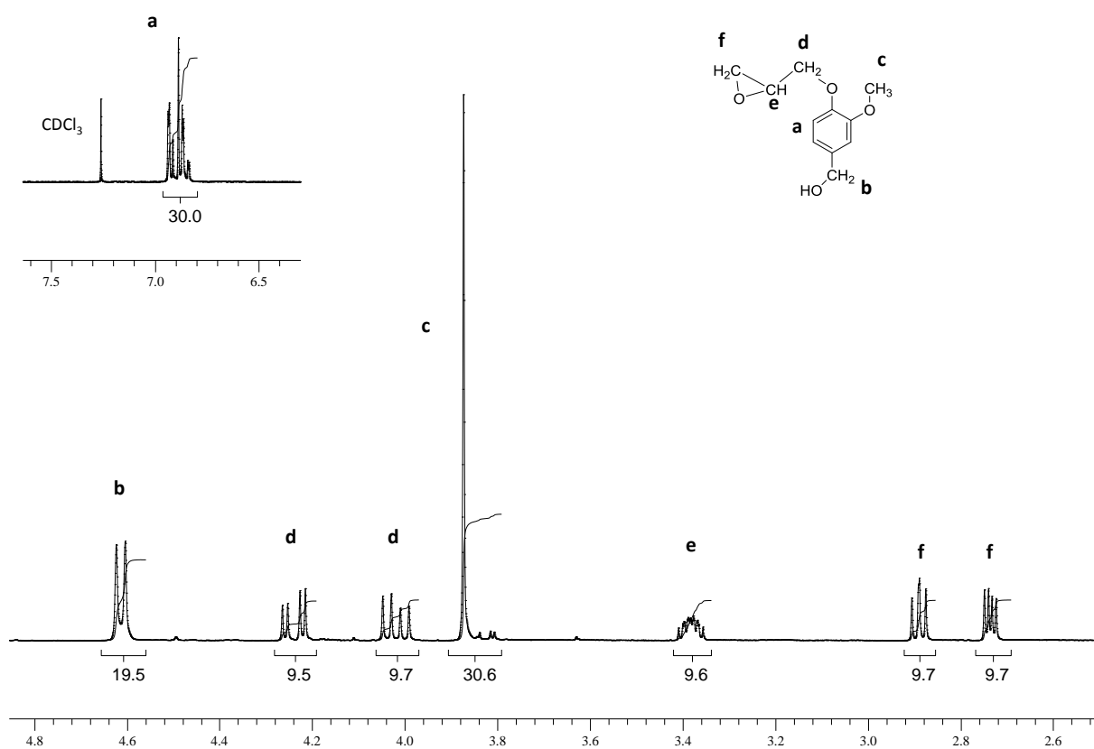
Figure 4: ^1\text{H} NMR spectrum of hydrochloride closure at room temperature.
