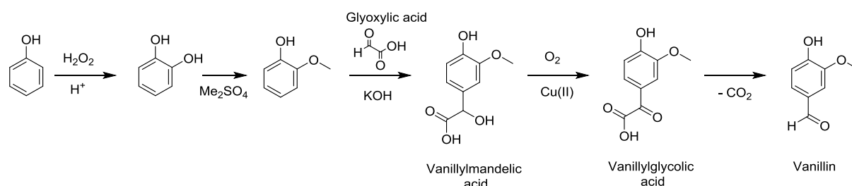
Figure S1: Solvay process of vanillin production from phenol
