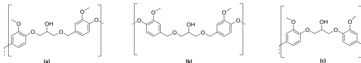
Scheme 6 : Structure of the oligomeric sequences obtained.
