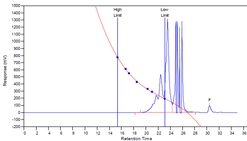
Figure S2: GPC Chromatogram of diepoxidized vanillin.
