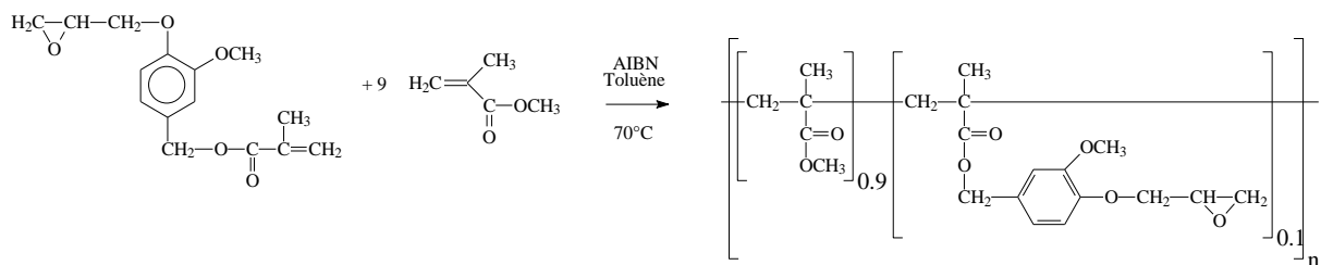
Scheme 7 : Copolymer synthesis of methacrylated glycidyl vanillin and MMA monomers.
