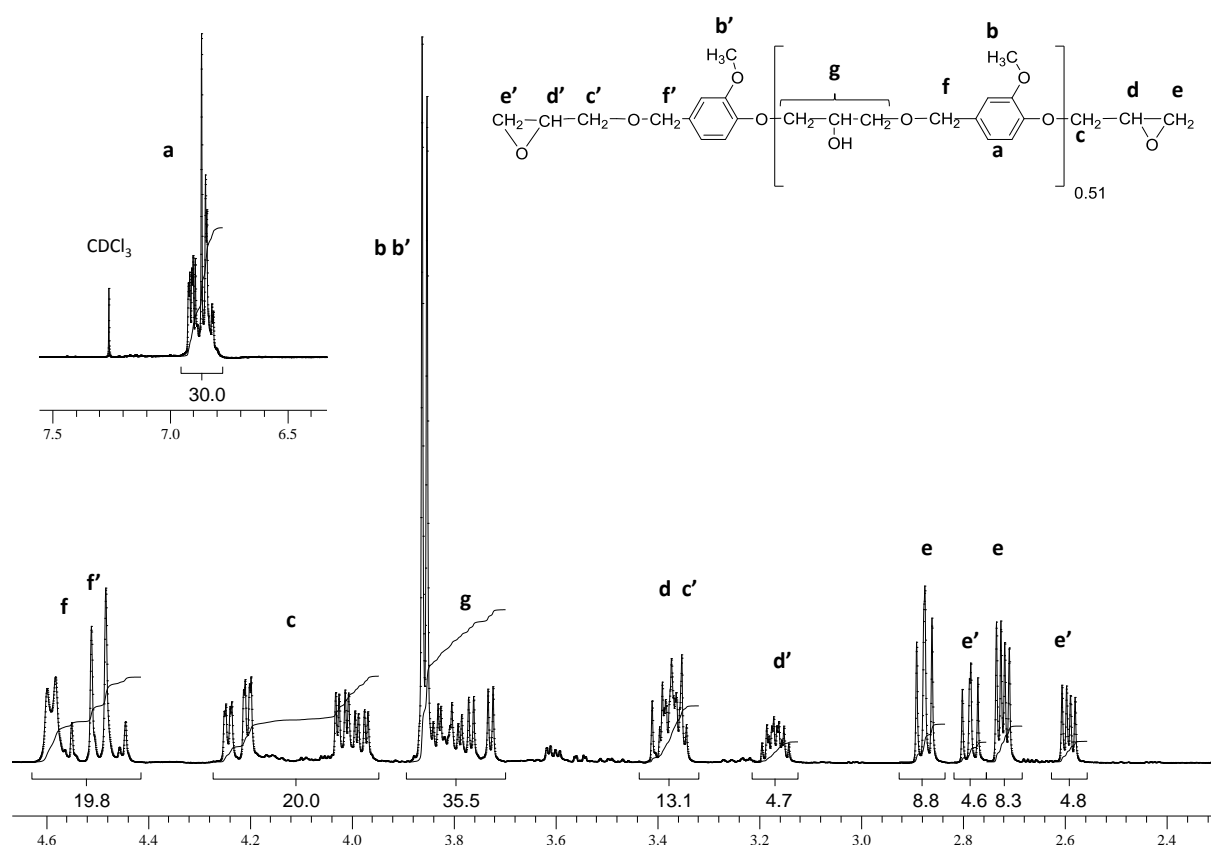
Figure 1: ^1\text{H} NMR Spectra of oligomeric diglycidylated of vanillyl alcohol (DGEVA).
