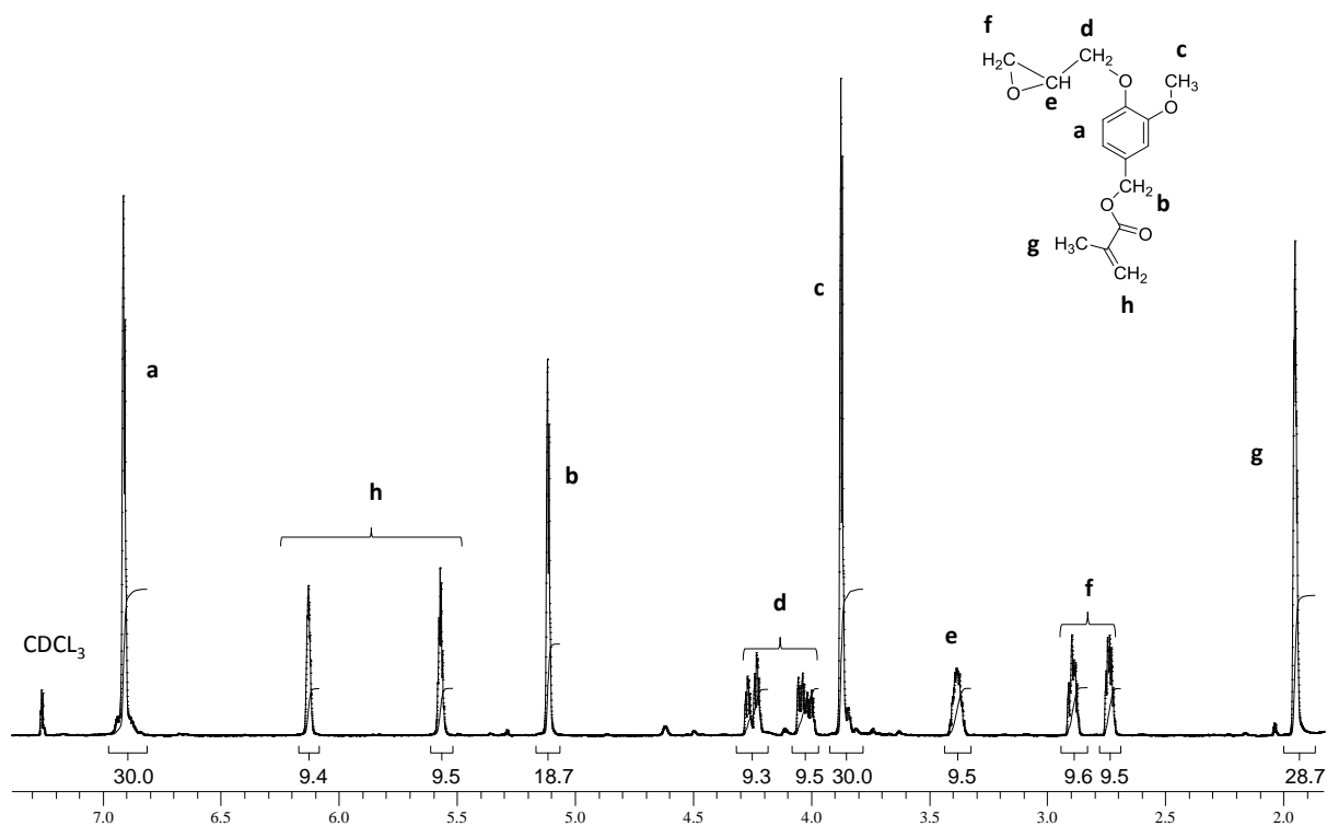
Figure 5 : ^1\text{H} NMR spectrum of methacrylated glycidyl vanillin .
