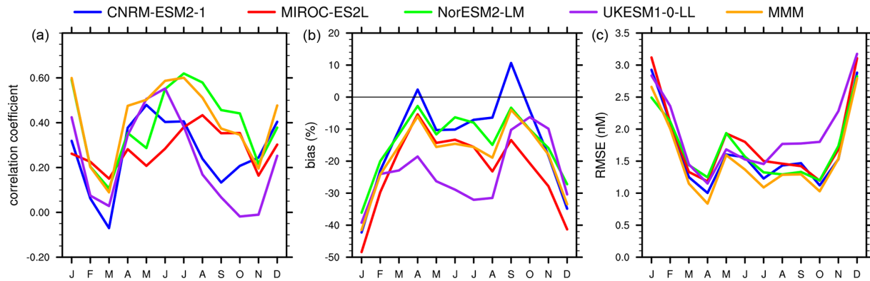
Figure 4. Monthly mean statistics of surface ocean DMS concentration. (a) Spatial correlations between a model and L11, (b) biases (in percentage of L11), and (c) RMSE (nM). A 0% bias line is drawn for visual aid. Model diagnostics are shown as in Fig. 1. The values are provided in Table S1 in the Supplement. The same metrics computed against G18 and W20 are plotted in Fig. S4.
