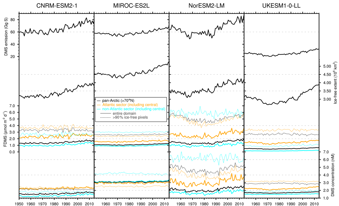
Figure 14. From top to bottom in each column are time series (1950–2014) of May–August values of integrated DMS emission (Gg S), mean ice-free extent ( 10^6 km 2 ), area-weighted mean DMS flux ( \mu\text{mol m}^{-2} \text{d}^{-1} ), and area-weighted mean DMS concentrations (nM). The same four months (May to August) and the same regions as those of Galí et al. (2019) are shown for the CMIP6 models in the four columns: black lines for pan-Arctic ( >70^\circ\text{N} ), cyan lines for non-Atlantic sector (including central), and orange lines for Atlantic sector (including central). Solid lines are for values computed from all pixels of a given region. Dashed lines are for DMS fluxes and DMS concentrations computed only from >90\% ice-free pixels of a given region, as in Galí et al. (2019). Grey dotted lines are visual aids to ease the comparison between models.
