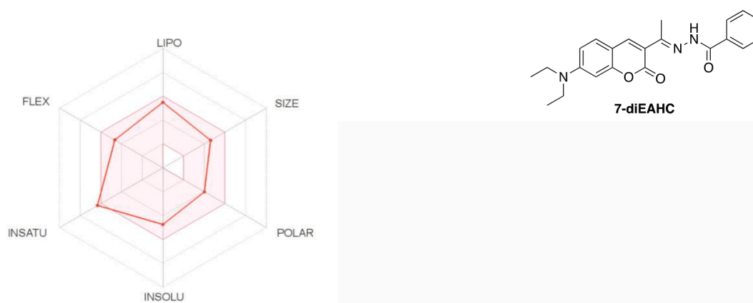
Fig. 4. Bioavailability radar related to the physicochemical properties of compound 7-diEAHC . The pink colored zone is the suitable physicochemical space for oral bioavailability. LIPO (Lipophilicity): -0.7 < \text{Log P} < +5.0 ; SIZE: 150 \text{ g/mol} < \text{MW} < 500 \text{ g/mol} ; POLAR (Polarity): 20 \text{ \AA}^2 < \text{tPSA} < 130 \text{ \AA}^2 ; INSOLU (Insolubility): -6 < \text{Log S} < 0 ; INSATU (Insaturation): 0.25 < \text{Fraction Csp}^3 < 1 ; FLEX (Flexibility): 0 < \text{Number rotatable bonds} < 9 .
