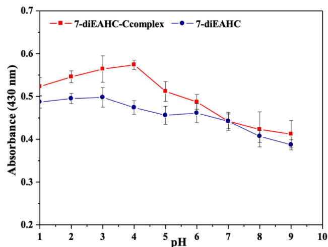
Fig. 6. Effect of pH on the free and microencapsulated 7-diEAHC.
