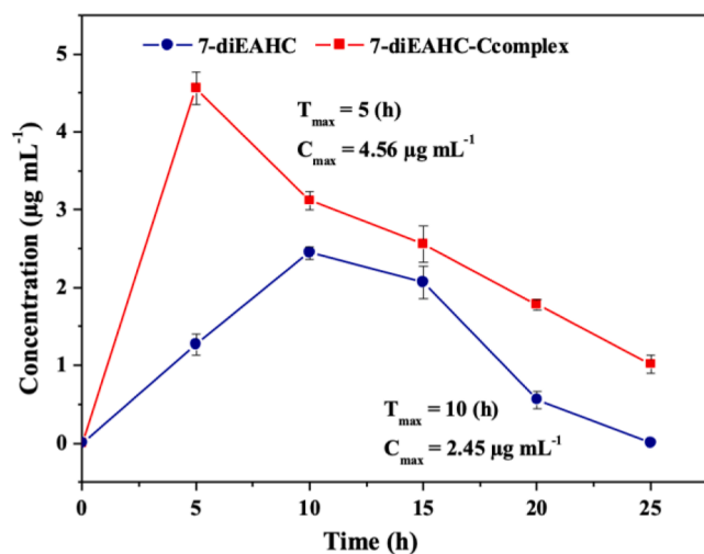
Fig. 9. Variation concentration in rat plasma after oral administration of free 7-diEAHC and encapsulated 7-diEAHC with \beta -CD. Data were represented as mean \pm SD, (n = 5).
