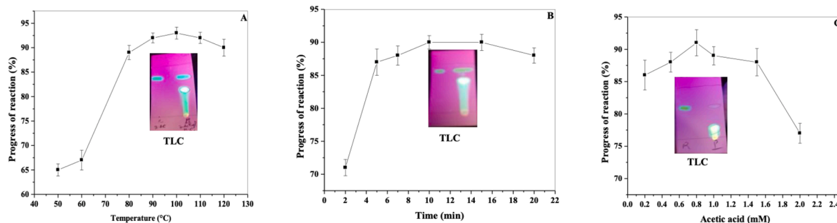
Fig. 2. Effect of temperature (A), reaction time (B) and % mol. of acetic acid (C) on the progress of reaction. Data are the mean \pm SD ( n = 3 ).
