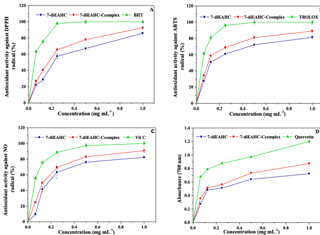
Fig. 8. In vitro antioxidant potential of free and encapsulated 7-diEAHC. Scavenging activity of free and encapsulated 7-diEAHC against DPPH (A), ABTS (B) and NO (C) radicals. Reducing power capacity of free and encapsulated 7-diEAHC against free Fe +3 (D). The data are presented as a mean value \pm SD.
