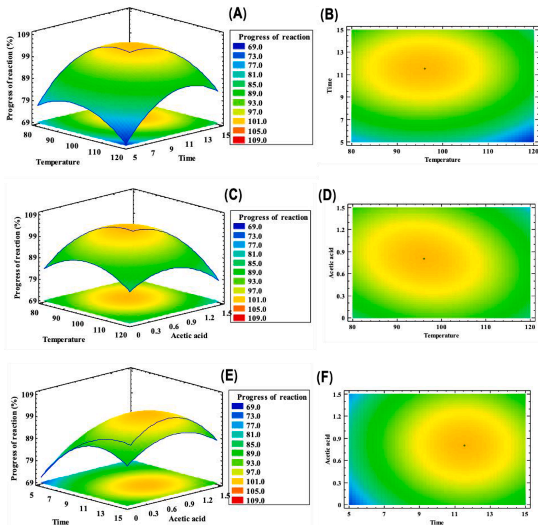
Fig. 3. Response surface (A, C and E) and contour plot (B, D and F) of different variables including the reaction temperature, the reaction time and AcOH % mol. in reaction medium for the second step of 7-diEAHC synthesis.
