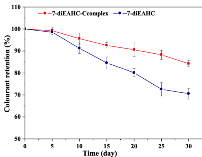
Fig. 5. Effect of natural light on the free and microencapsulated 7-diEAHC.
