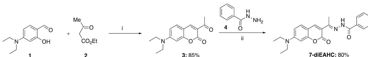
Scheme 1. Synthesis of ( E )- N' -(1-(7-(diethylamino)-2-oxo-2 H -chromen-3-yl)ethylidene)benzohydrazide ( 7-diEAHC ). Reagents and reaction conditions: i) piperidine, EtOH, reflux, 35 min. ii) AcOH, EtOH, MWI, 100 °C, 10 min.
