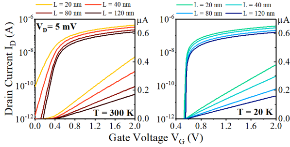
Figure 7. Simulated I_D(V_G) for different L_G at T = 300 K (a) and T = 20 K (b).
