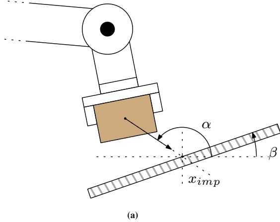
Fig. 5: Defining various impact scenarios. (a) The impact approach angle \alpha , impact surface inclination \beta , and desired impact location x_{imp} are defined. (b) A snapshot of experiments where the robot is impacting the impact platform for an expected (top) and unexpected (bottom) impact scenario at starting time t_0 , first detected impact time t_1 , and end time t_f .
