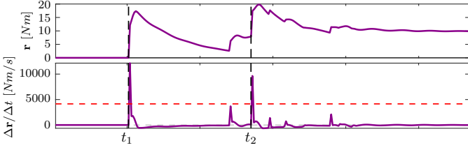
Fig. 4: The momentum observer residual and its numerical derivative during a simulated simultaneous impact sequence. The dashed red line is the impact detection threshold \mathbf{r}_b . By adjusting \mathbf{r}_b , smaller impacts that are of lesser interest for the classification method can be included or excluded.
