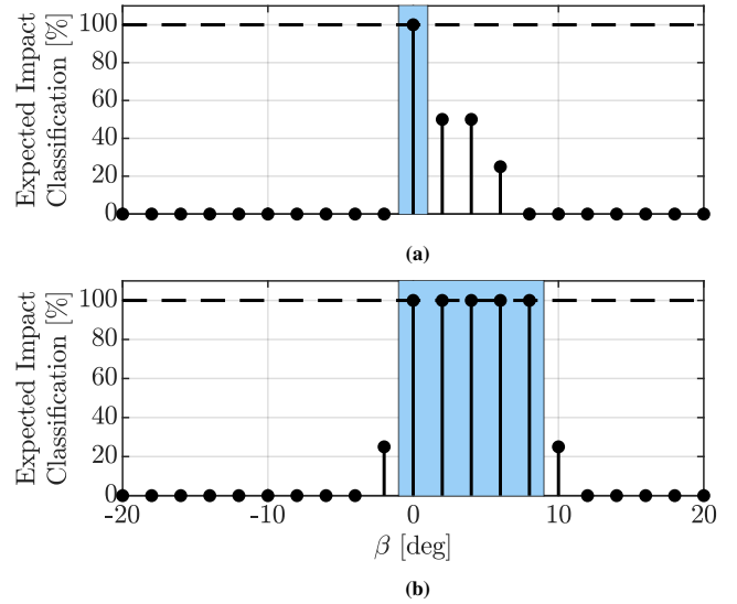
Fig. 8: Expected impact classification percentage for simultaneous impact scenarios on the experimental setup tuned for varying sensitivities. The blue band represents the range of inclinations that are always classified as expected. (a) The tuned classifier classifies \beta = 0 as expected. (b) The tuned classifier classifies \beta \in \{0, \dots, 8\} as expected.
