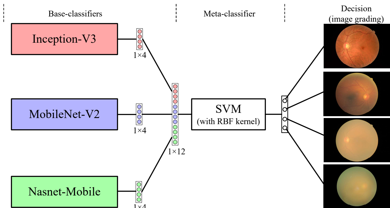
Figure 4. Processing pipeline of ensemble learning framework for cataract grading
