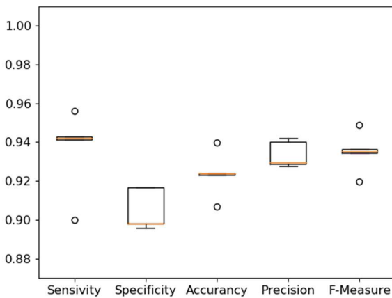
Figure 6. Performance visualization of cataract grading using box plots
