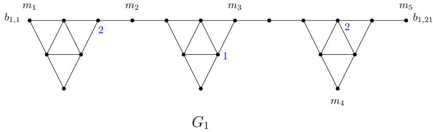
Fig. 4: G_1 is a connected chordal graph with \gamma_b(G_1) = 5 and \text{mp}(G_1) = 5 . M_1 = \{m_i : 1 \leq i \leq 5\} is a multipacking of size 5.
