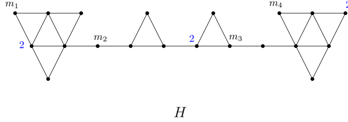
Fig. 3: H is a connected chordal graph with \gamma_b(H) = 6 and \text{mp}(H) = 4
