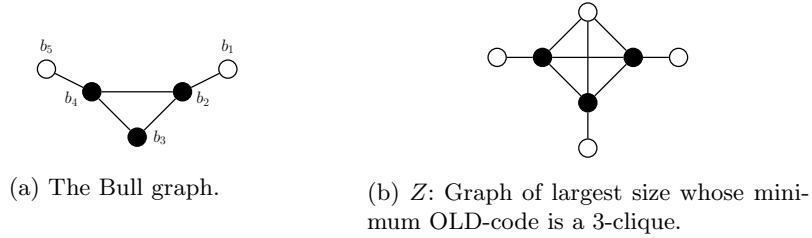
Fig. 5: The black vertices constitute a minimum respective code of each graph.
