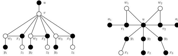
(a) Block graph H_3 whose LD-number attains the upper bound in Theorem 4. (b) Block graph G_{2,3} whose OLD-number attains the upper bound in Theorem 6.
