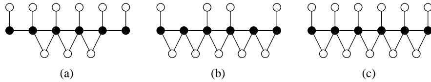
Fig. 6: Extremal cases where the lower bounds are attained, black vertices form a minimum (a) ID-code, (b) OLD-code, (c) LD-code.
