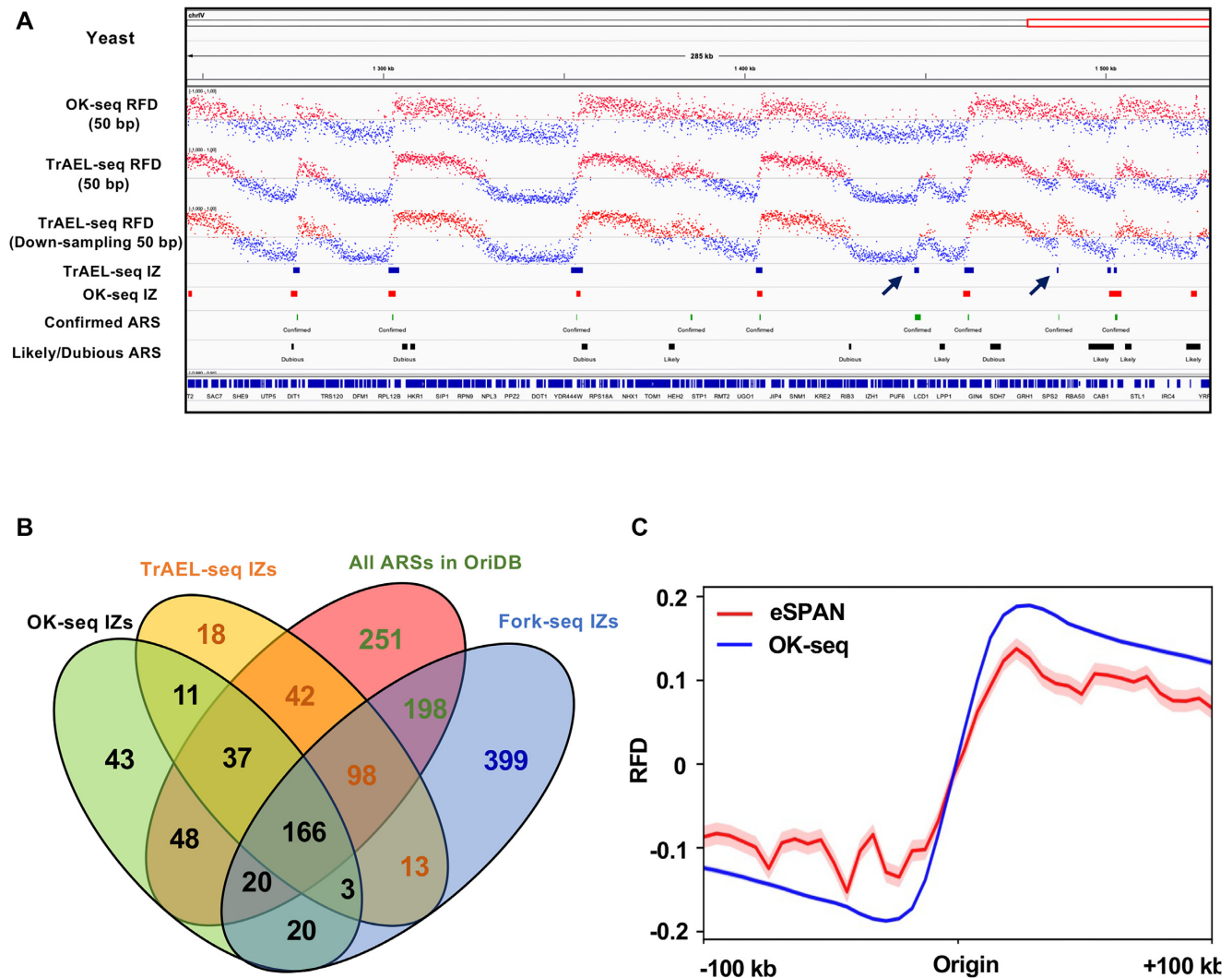
Figure 7. Genome-wide RFD profiles obtained using TrAEL-seq and eSPAN datasets. (A) RFD profiles and the corresponding IZs (50 bp bin size) from yeast OK-seq and TrAEL-seq datasets (11). The known yeast origins (ARS) were downloaded from OriDB. Arrows indicate two IZs (chrIV:1447102–1448300, chrIV:1486452–1486950) identified in the TrAEL-seq dataset but not in the OK-seq dataset. (B) Venn diagram showing the overlap between OK-seq IZs ( n = 348 ), TrAEL-seq IZs ( n = 380 ), FORK-seq initiation events ( n = 4964 ), and known origins (ARS) from OriDB ( n = 829 ); overlap means that the closest distance between the centre of an IZ and of an ARS is <2 kb. When origins in one dataset overlapped with several origins in the other datasets, only one number was provided with the following priority order: OK-seq > TrAEL-seq > OriDB > FORK-seq. It should be noted that there are more origins unique to FORK-seq because this is a single-molecule technique that allows identifying also initiation events with very low frequency. (C) Metagene average RFD profiles computed using the OK-seq and eSPAN datasets from mouse embryonic stem cells (8). The mean and standard error bands are shown only for the eSPAN dataset because the standard error bands for the OK-seq dataset were too narrow to be seen.
