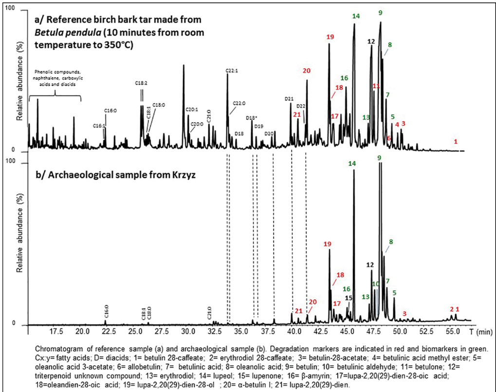
Figure 8. Chromatogram of the reference sample of birch bark tar (a) and archaeological sample from Krzyz (b) (figure by M. Rageot, A. Mazuy and M. Regert).
