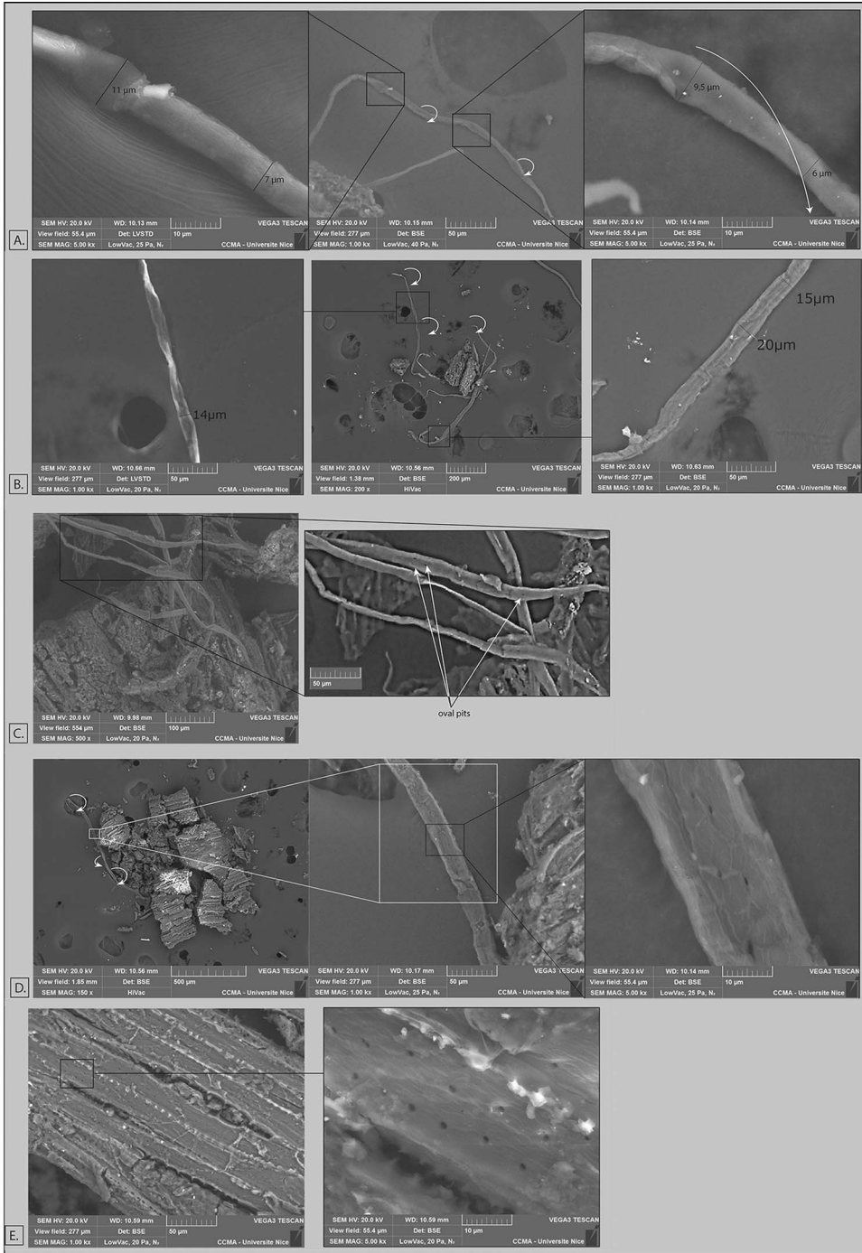
Figure 7. SEM micrographs of the ligature sample (A–D) and reference poplar bast (E) (figure by C. Cheval, A. Henry and F. Orange).
