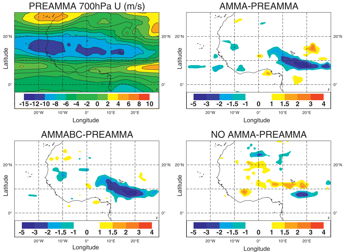
FIG. 7. The 700-hPa zonal wind ( m s^{-1} ) averaged over the period 1 Aug–14 Sep, at 1200 UTC, for (top left) PREAMMA, and the differences between (top right) AMMA and PREAMMA, (bottom left) AMMABC and PREAMMA, and (bottom right) NOAMMA and PREAMMA.
