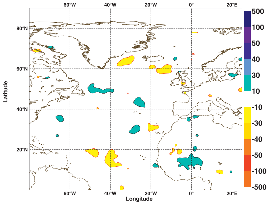
FIG. 12. Differences in RMS errors (m) between the AMMABC and PREAMMA forecasts. The errors are computed with respect to the ECMWF analysis, for the geopotential at 500 hPa at 24-h range, over the period 1 Aug–14 Sep 2006.
