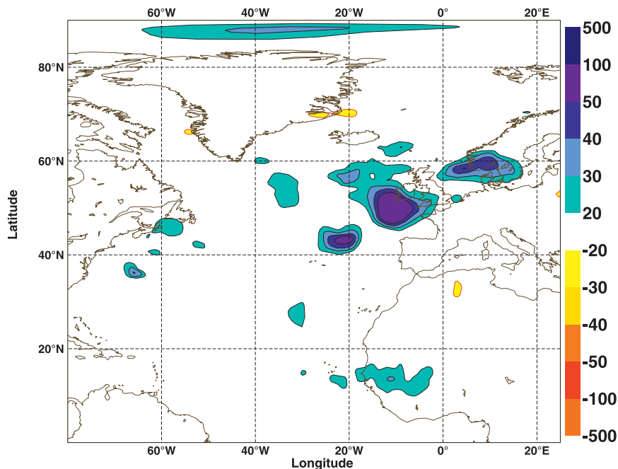
FIG. 13. Differences in RMS errors (m) between the AMMABC and PREAMMA forecasts. The errors are computed with respect to the ECMWF analysis, for the geopotential at 500 hPa at 48-h range, over the period 1 Aug–14 Sep 2006.
