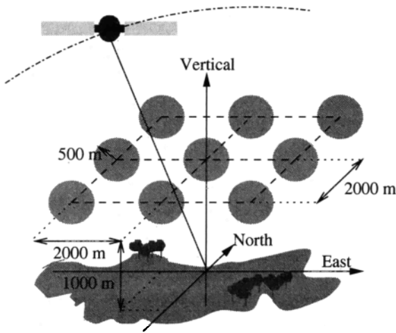
Figure 1. View of the simulated atmospheric inhomogeneities (1 km-size eddies).
