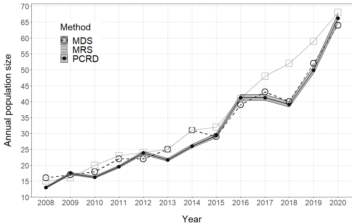
Figure 2: Variation in the annual population size of the Pyrenean brown bear from 2008 to 2020, estimated from Bayesian Pollock's robust design capture-recapture approach (PCRDR, black full circles and black full line, with the associated 95% credible interval in grey), compared to the Minimum Retained population Size (MRS, grey open squares and grey full line) and Minimum Detected population Size (MDS, black open circles and black dashed line) values.
