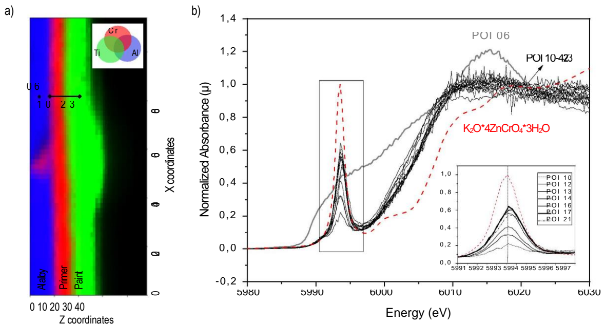
Figure 6. LA298 cross-section sample: a) XRF (Cr, Ti, Al) map with POI 06 (in the Al alloy) and POIs from 10 to 23; b) Normalised XANES spectra across the Al/primer interface: POI 06 (Al alloy), POI 10-POI 11 (interface); POI 14 (in the middle of the layer) plotted together with that of the reference Zn yellow (dashed line); inset: close-up view of the pre-edge peak.
