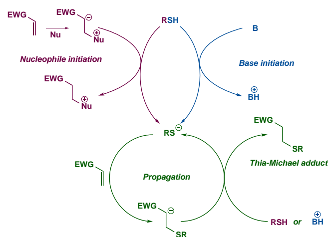
Scheme 1. Thia-Michael addition : nucleophile-initiated mechanism (top left) and base-catalyzed mechanism (top right).
