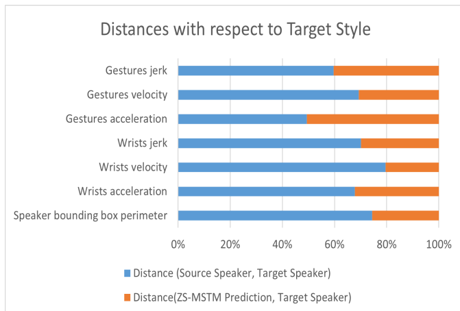
(b) Style transfer from unseen speakers
