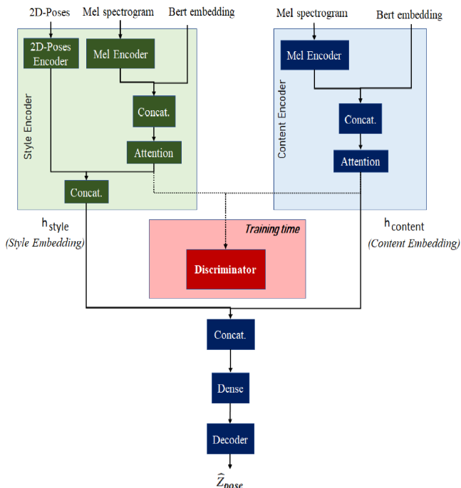
Fig. 1: ZS-MSTM model architecture.
