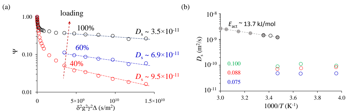
Fig. 5. (a) Attenuation \Psi of the spin echo signal at -20^\circ\text{C} for \Delta = 10 ms as a function of the gradient strength, g , measured by PFG NMR for cyclohexane adsorbed in a mesoporous FAU (the NaOH/Si molar ratio is 0.1). The porosity is partially or totally filled with a filling ratio increasing from 40–100% (a loading of 40% means that only the microporosity is filled with some adsorbed molecules at the mesopore surface, while a loading of 100% means that both the microporosity and mesoporosity are filled with cyclohexane). These measurements were performed for an observation time \Delta = 10 ms. The graph also reports the self-diffusivity D_s obtained from such attenuation curves. (b) Effect of temperature on the self-diffusivity, D_s , as measured by PFG NMR for cyclohexane adsorbed in mesoporous FAU: (green circles) NaOH/Si = 0.1, (red circles) NaOH/Si = 0.088, and (blue circles) NaOH/Si = 0.075. The grey and white circles are the self-diffusivity for bulk cyclohexane. All data for confined cyclohexane, which were taken for T = -20, 0, and 15^\circ\text{C} , correspond to a loading where the microporosity is completely filled with some adsorbed molecules at the mesopore surface (filling ratio 40%).
