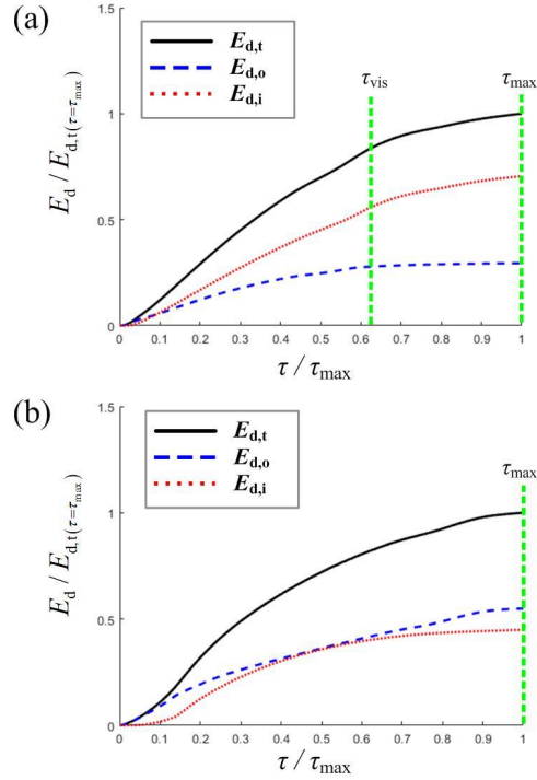
Fig. 14. Comparisons of two energy dissipation quantities: the capillary-wave-induced dissipation ( E_{d,o} ) and the near wall dissipation ( E_{d,i} ). We = 3.5 . (a) hydrophilic surface ( \theta_{eqi} = 20^\circ ), and (b) hydrophobic surface ( \theta_{eqi} = 125^\circ ).
